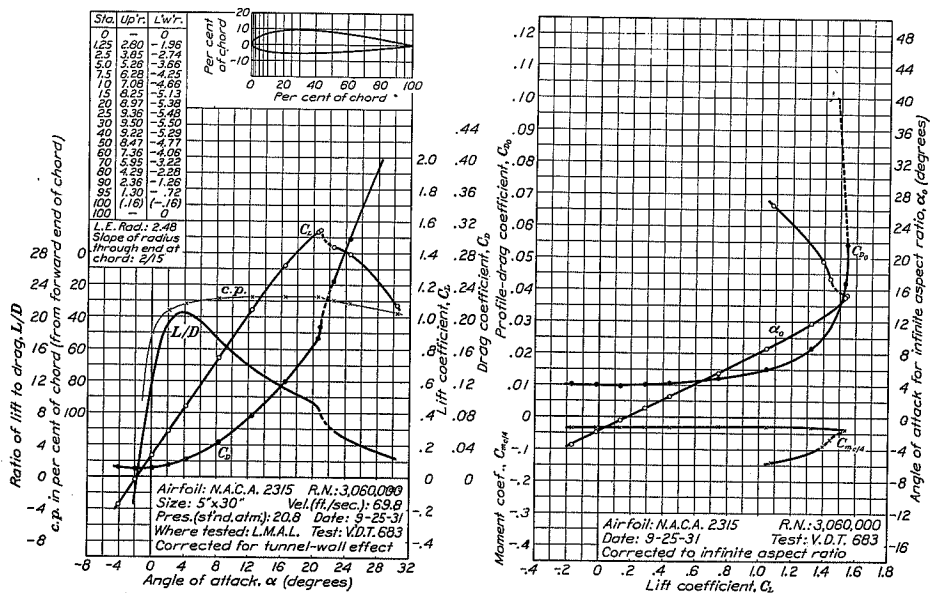
FIGURE 15.—N.A.C.A. 2315 airfoil.
