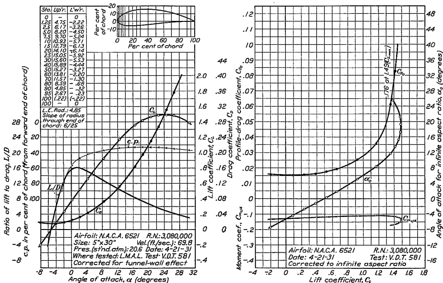
FIGURE 69.—N.A.C.A. 6521 airfoil.
