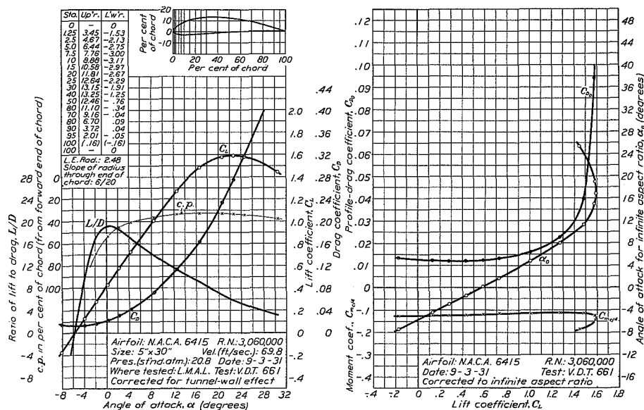
FIGURE 61.—N.A.C.A. 6415 airfoil.
