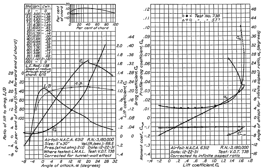
FIGURE 54.—N.A.C.A. 6312 airfoil.
