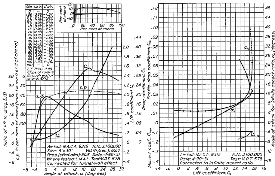
FIGURE 55.—N.A.C.A. 6315 airfoil.
