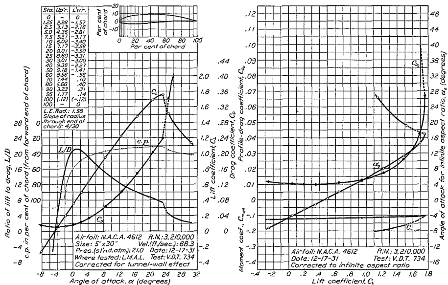
FIGURE 49.—N.A.C.A. 4612 airfoil.
