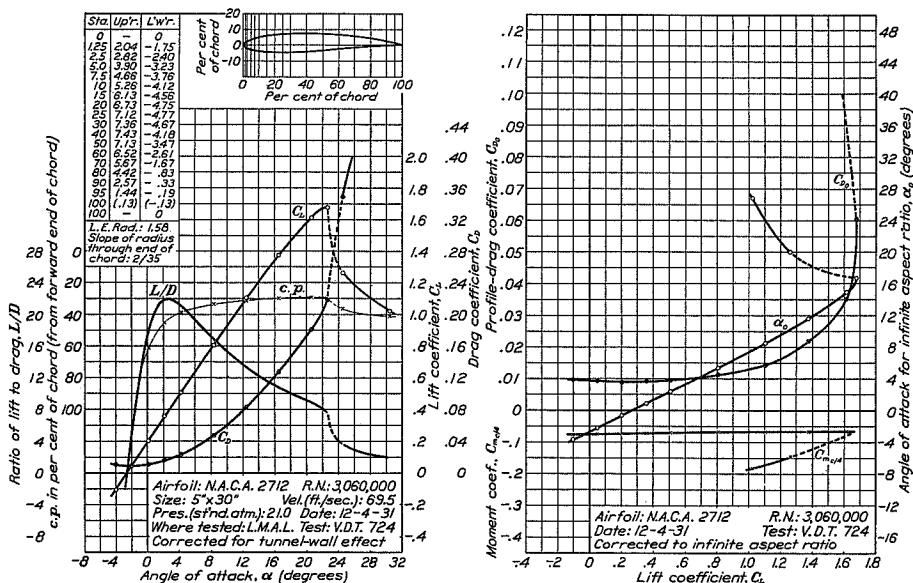
FIGURE 29.—N.A.C.A. 2712 airfoil.
