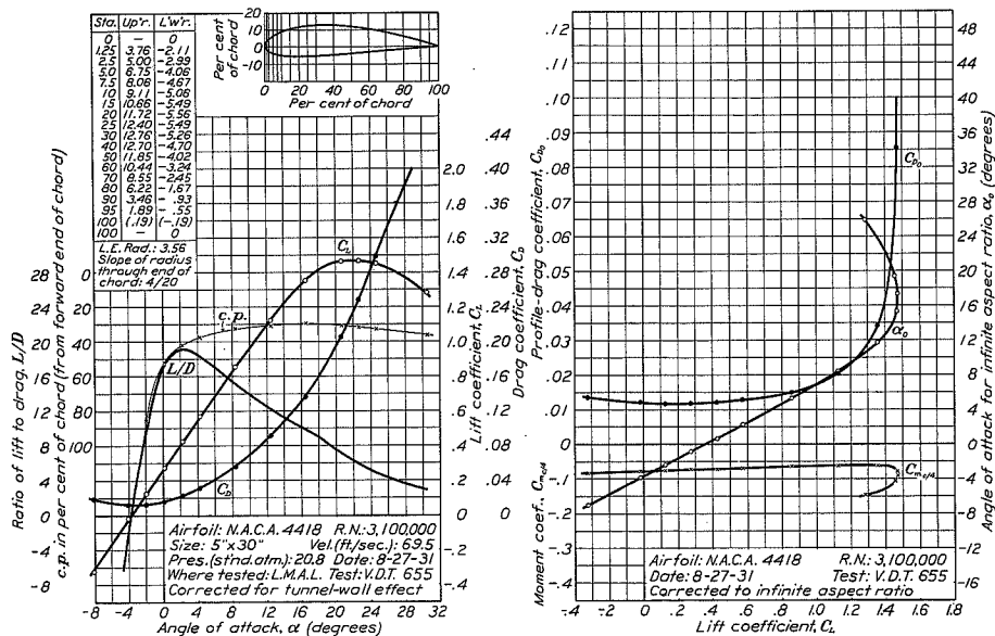
FIGURE 41.—N.A.C.A. 4418 airfoil.
