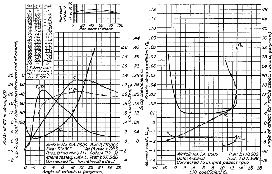
FIGURE 64.—N.A.C.A. 6506 airfoil.
