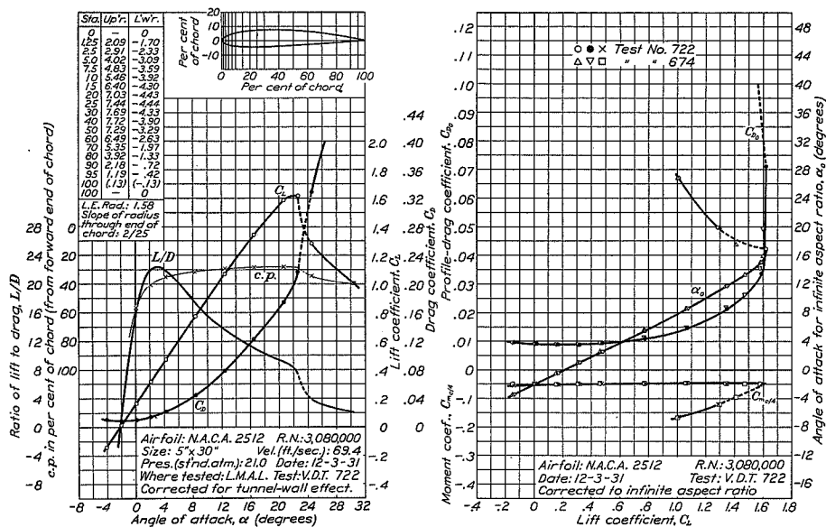
FIGURE 24.—N.A.C.A. 2512 airfoil.
