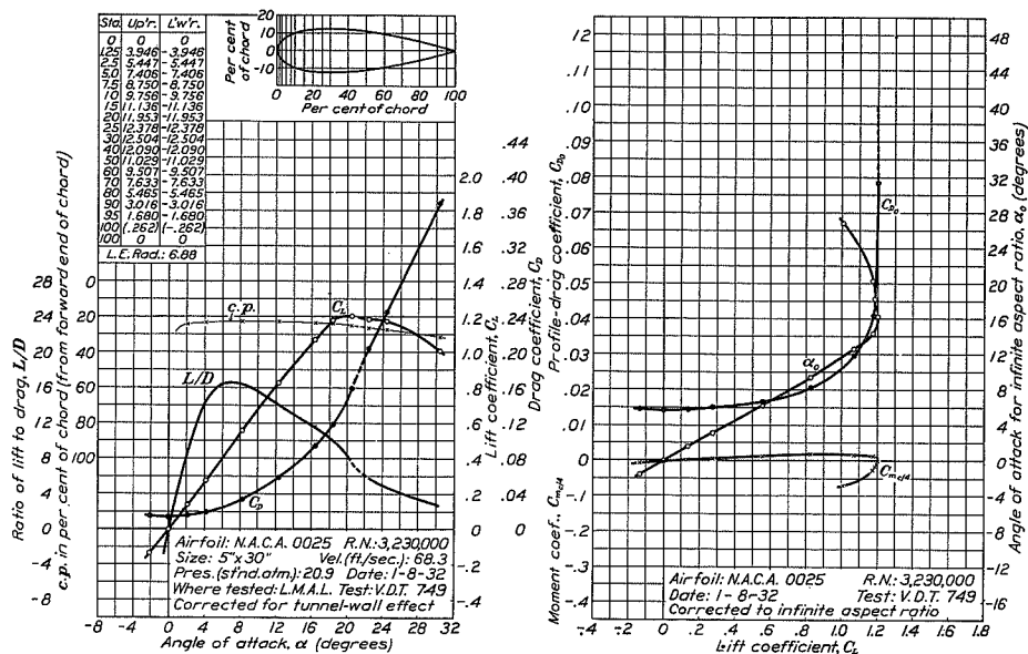
FIGURE 10.—N.A.C.A. 0025 airfoil.
