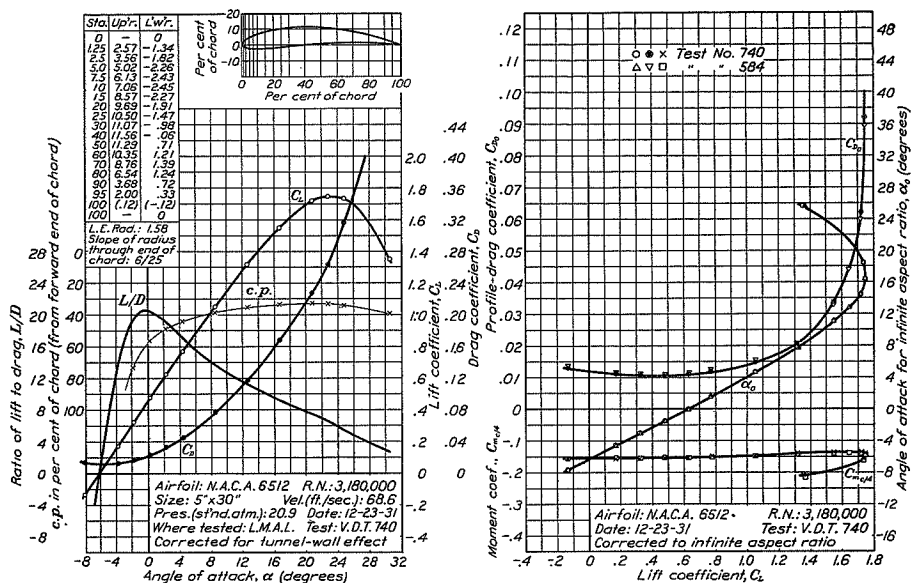
FIGURE 66.—N.A.C.A. 6512 airfoil.
