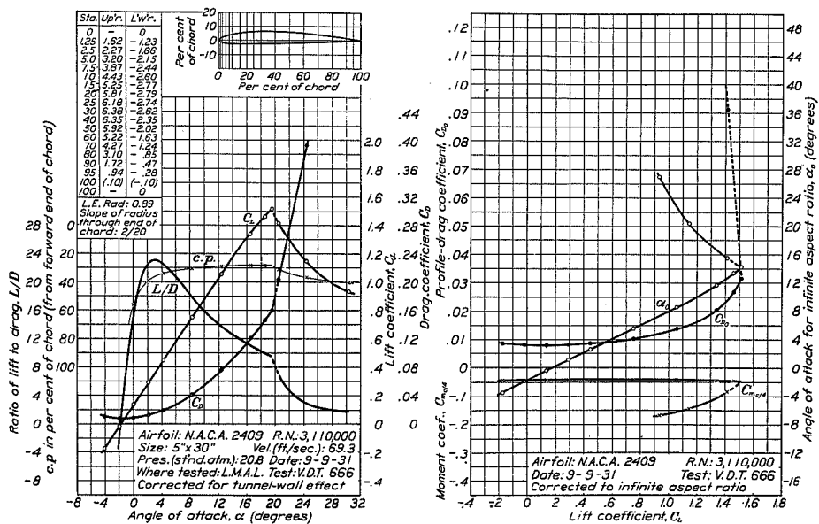
FIGURE 17.—N.A.C.A. 2409 airfoil.
