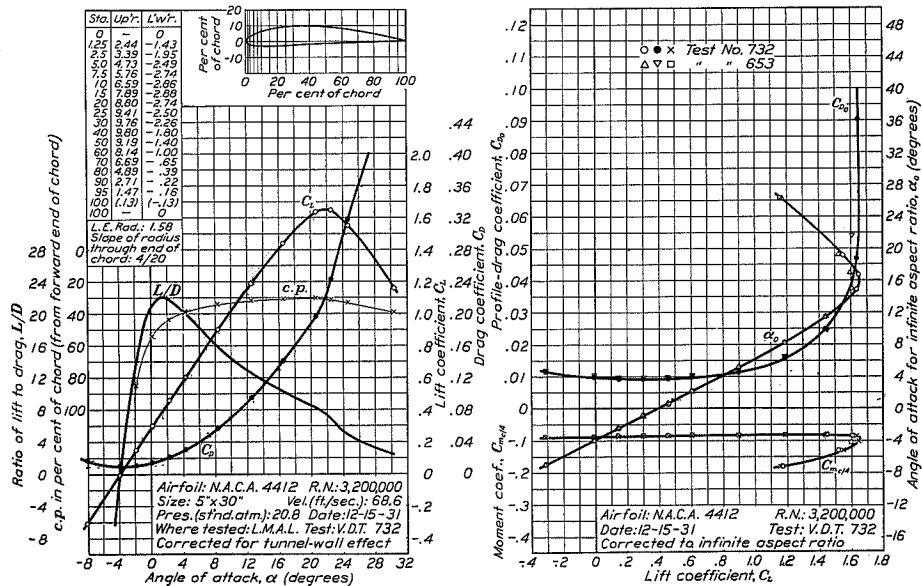
FIGURE 39.—N.A.C.A. 4412 airfoil.
