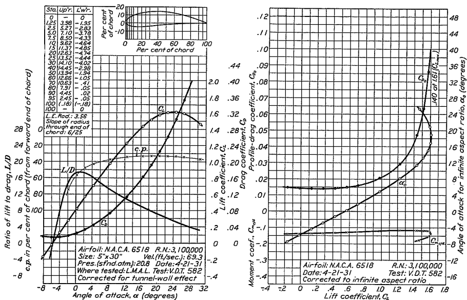
FIGURE 68.—N.A.C.A. 6518 airfoil.
