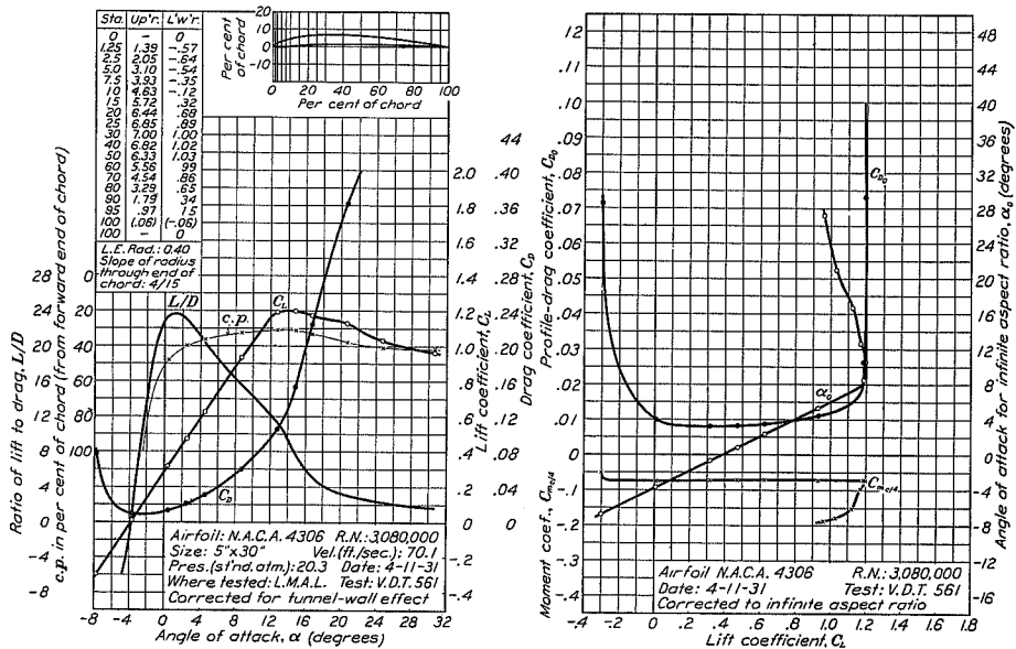
FIGURE 31.—N.A.C.A. 4306 airfoil.
