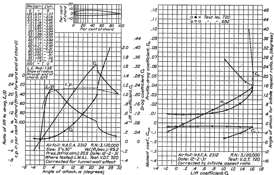
FIGURE 14.—N.A.C.A. 2312 airfoil.
