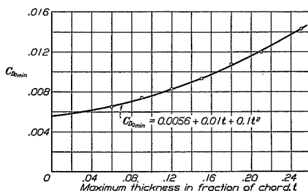
FIGURE 91.—Variation of minimum profile drag with thickness for the symmetrical airfoils.
