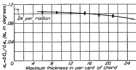
FIGURE 81.—Variation of lift-curve slope with thickness.
