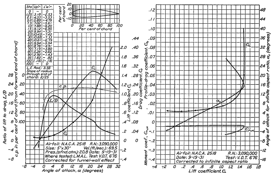
FIGURE 26.—N.A.C.A. 2518 airfoil.
