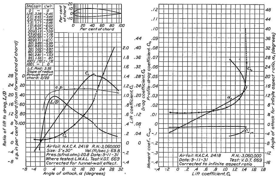
FIGURE 20.—N.A.C.A. 2418 airfoil.
