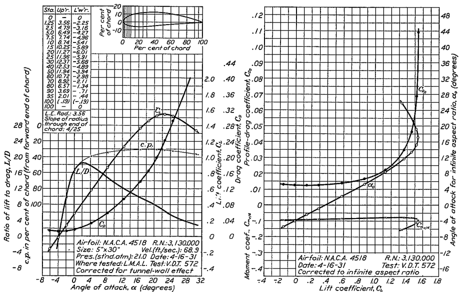
FIGURE 47.—N.A.C.A. 4518 airfoil.
