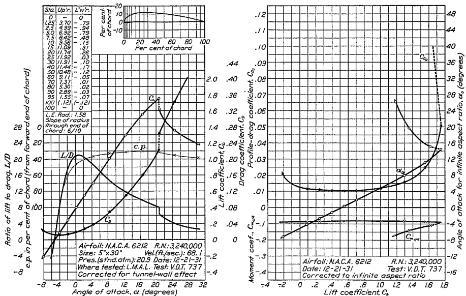
FIGURE 51.—N.A.C.A. 6212 airfoil.
