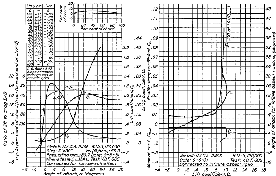
FIGURE 16.—N.A.C.A. 2406 airfoil.
