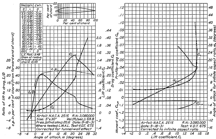
FIGURE 25.—N.A.C.A. 2515 airfoil.
