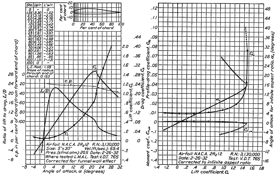
FIGURE 79.—N.A.C.A. 2R212 airfoil.
