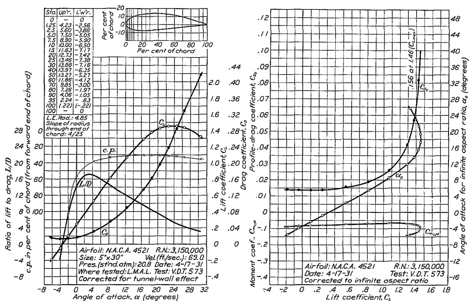
FIGURE 48.—N.A.C.A. 4521 airfoil.
