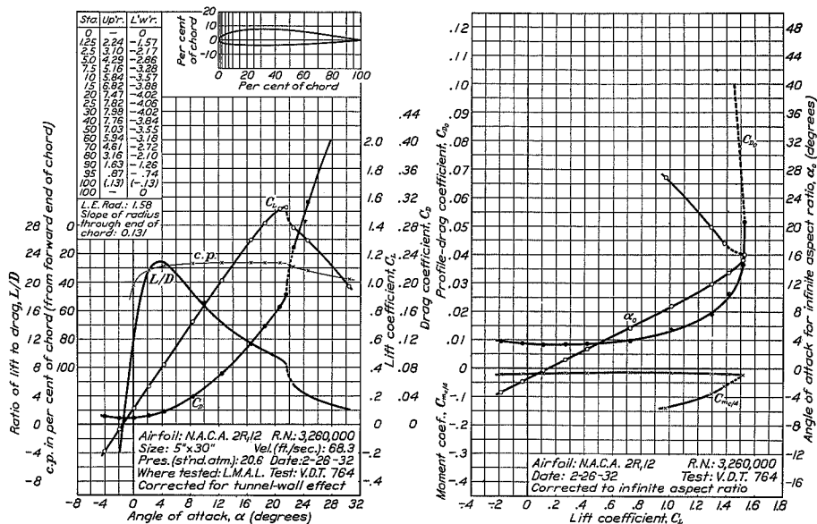
FIGURE 78.—N.A.C.A. 2R12 airfoil.
