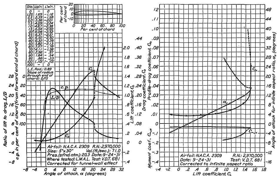
FIGURE 13.—N.A.C.A. 2309 airfoil.
