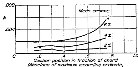
FIGURE 92.—Increase in minimum profile drag due to camber. Results for 12 percent thick airfoils. Values of k for equation C_{D_{0min}} = k + 0.0056 + 0.01t + 0.1t^2 , where k is the increase in C_{D_{0min}} due to camber and t is the maximum thickness in fraction of chord.
