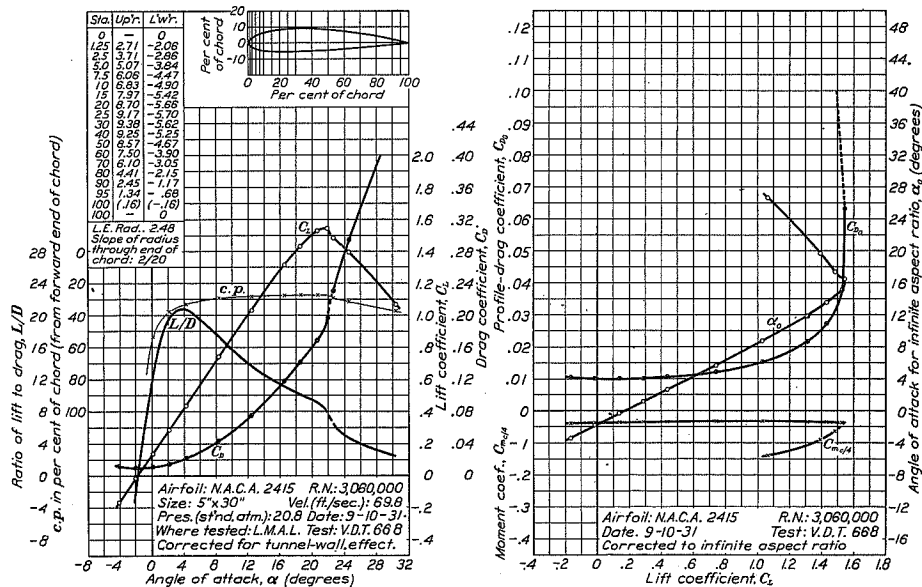
FIGURE 19.—N.A.C.A. 2415 airfoil.
