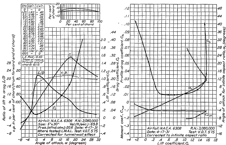
FIGURE 52.—N.A.C.A. 6306 airfoil.
