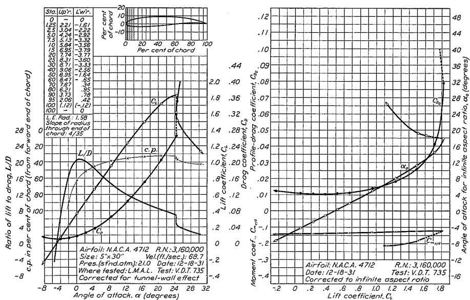
FIGURE 50.—N.A.C.A. 4712 airfoil.
