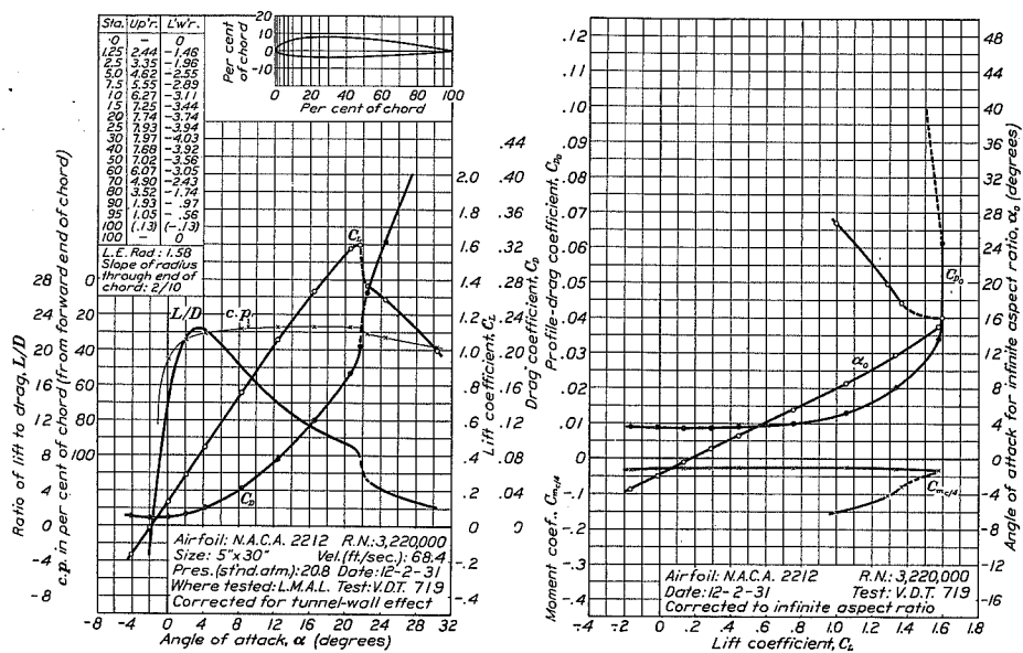
FIGURE 11.—N.A.C.A. 2212 airfoil.
