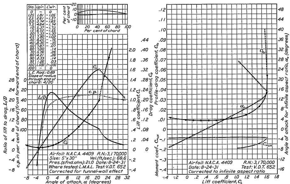
FIGURE 38.—N.A.C.A. 4409 airfoil.
