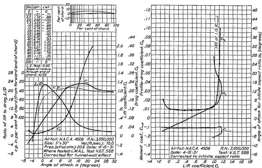
FIGURE 43.—N.A.C.A. 4506 airfoil.
