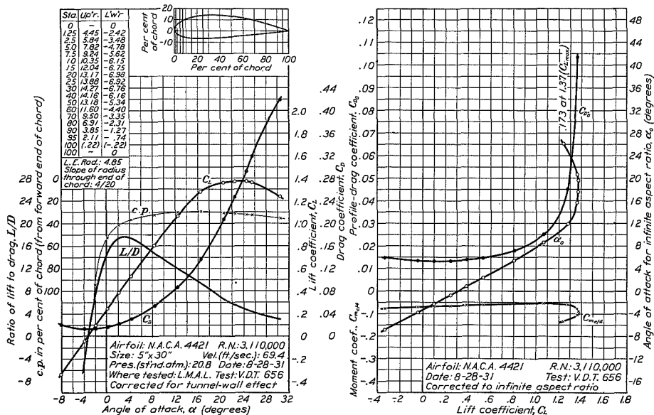
FIGURE 42.—N.A.C.A. 4421 airfoil.
