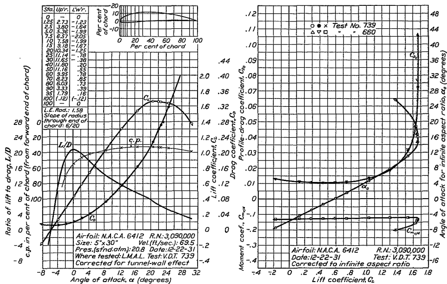
FIGURE 60.—N.A.C.A. 6412 airfoil.
