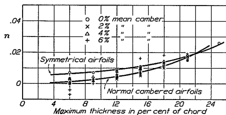
FIGURE 89.—Variation of position of constant moment with thickness. Values of n for equation C_{m_{c/4}} = C_{m_0} + nC_L . Results for airfoils having normal camber positions (0.3c to 0.5c).
