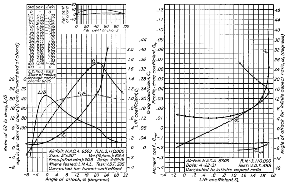
FIGURE 65.—N.A.C.A. 6509 airfoil.
