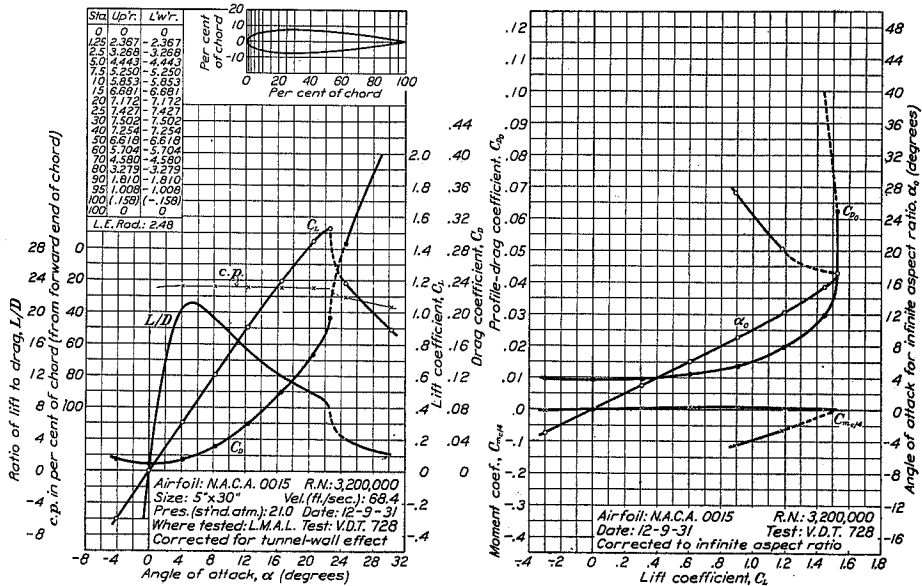
FIGURE 7.—N.A.C.A. 0015 airfoil.
