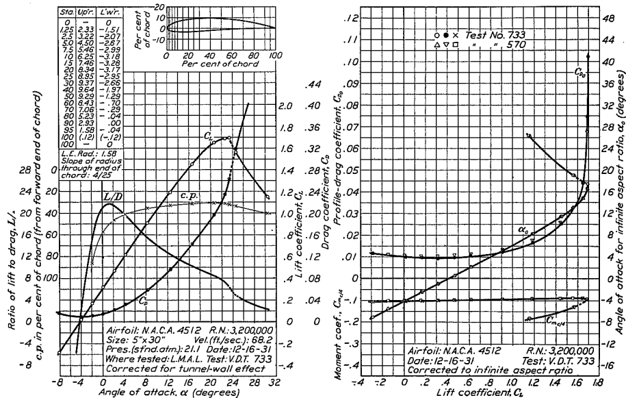
FIGURE 45.—N.A.C.A. 4512 airfoil.
