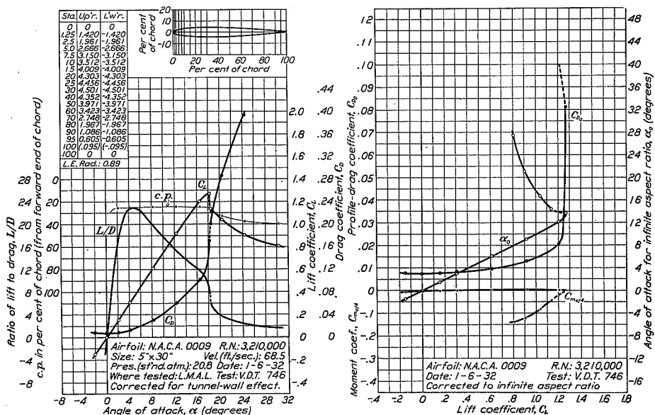
FIGURE 5.—N.A.C.A. 0009 airfoil.
