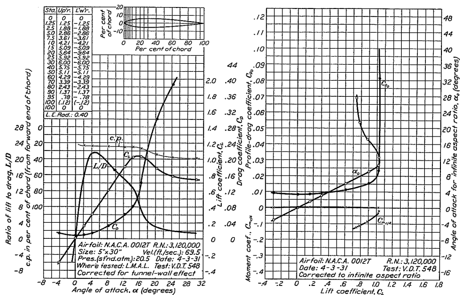
FIGURE 74.—N.A.C.A. 0012T airfoil.
