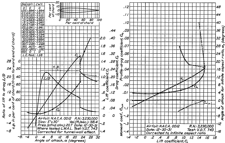
FIGURE 6.—N.A.C.A. 0012 airfoil.
