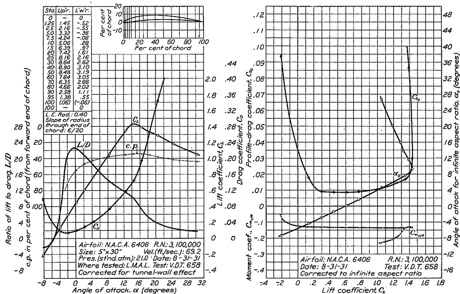
FIGURE 58.—N.A.C.A. 6406 airfoil.
