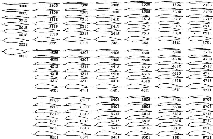
FIGURE 3.—N.A.C.A. airfoil profiles.
