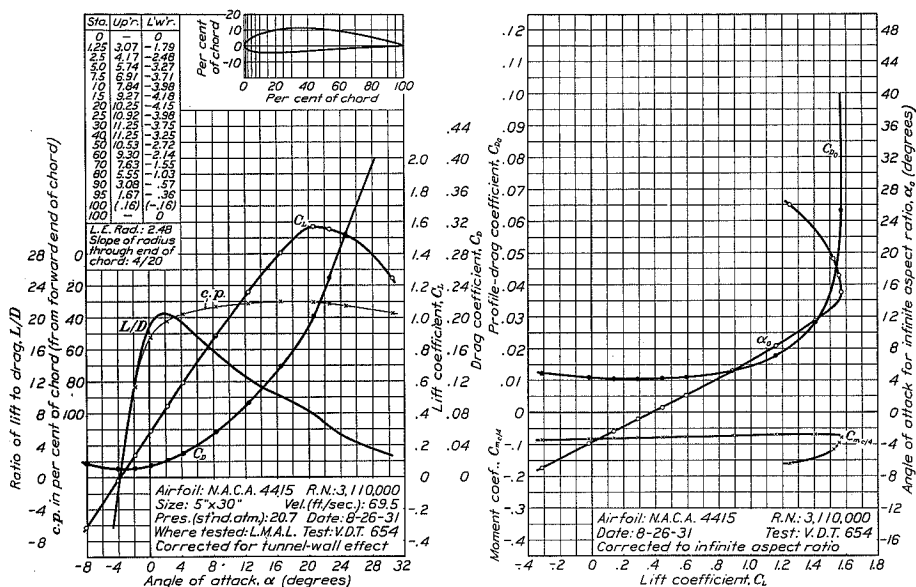
FIGURE 40.—N.A.C.A. 4415 airfoil.
