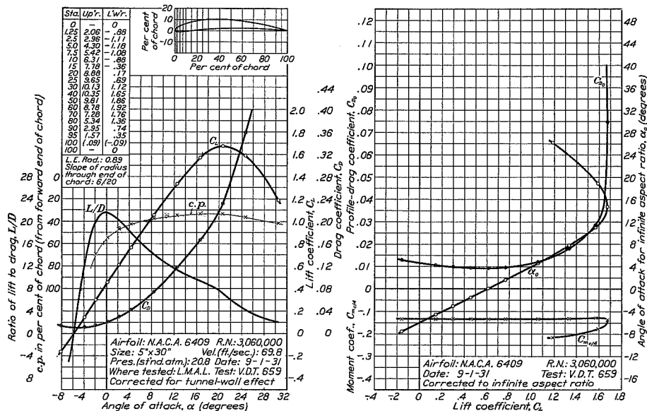
FIGURE 59.—N.A.C.A. 6409 airfoil.
