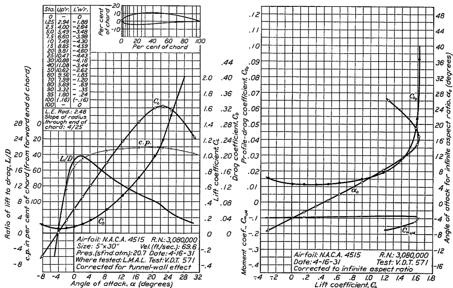
FIGURE 46.—N.A.C.A. 4515 airfoil.
