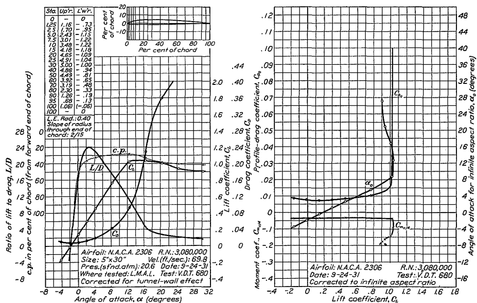
FIGURE 12.—N.A.C.A. 2306 airfoil.
