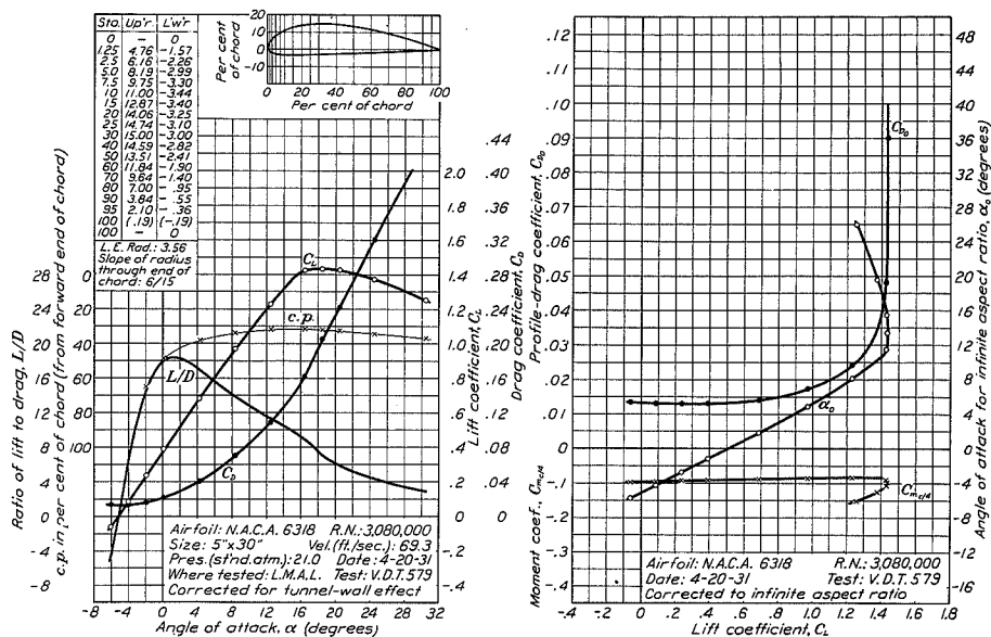
FIGURE 56.—N.A.C.A. 6318 airfoil.
