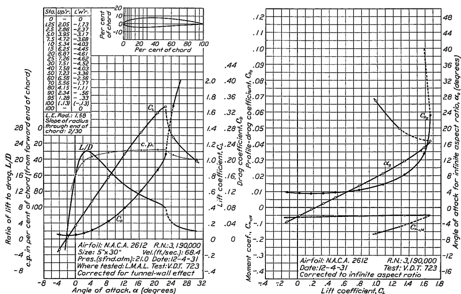
FIGURE 28.—N.A.C.A. 2612 airfoil.
