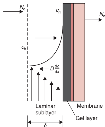
■ Figure 11.10 A concentration profile showing the formation of a gel layer on an ultrafiltration membrane. (From Schweitzer, 1979)
