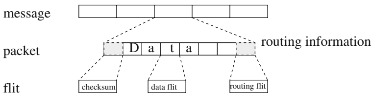
Fig. 2.29 Illustration of the partitioning of a message into packets and of packets into flits (flow control units)
