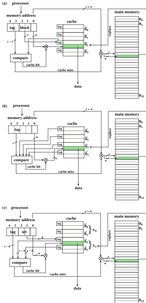
Fig. 2.33 Illustration of the mapping of memory blocks to cache blocks for a cache with m = 4 cache blocks ( r = 2 ) and a main memory with n = 16 memory blocks ( s = 4 ). Each block contains two memory words ( w = 1 ). (a) Direct mapped cache; (b) fully associative cache; (c) set associative cache with k = 2 blocks per set, using v = 2 sets ( d = 1 )
