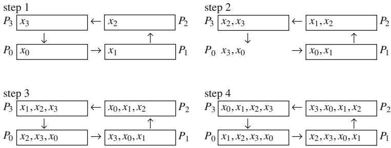
Fig. 5.2 Illustration for the collection of data in a logical ring structure for p = 4 processes
