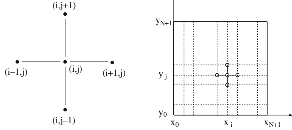
Fig. 7.8 Five-point stencil resulting from the discretization of the Laplace operator with a finite difference scheme. The computation at one mesh point uses values at the four neighbor mesh points
