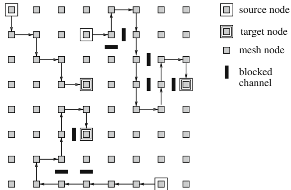
Fig. 2.23 Illustration of path selection for west-first routing in an 8 \times 8 mesh. The links shown as blocked are used for other message transmissions and are not available for the current transmission. One of the paths shown is minimal, the other two are non-minimal, since some of the links are blocked
