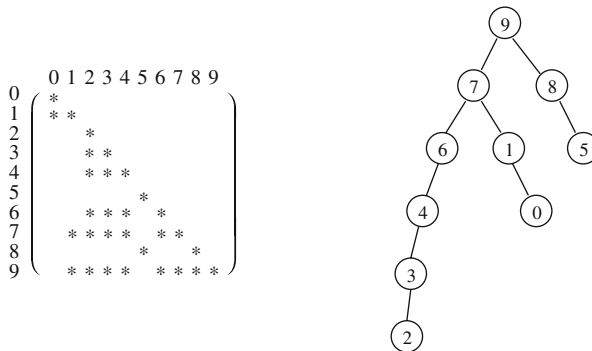
Fig. 7.23 Matrix L with supernodes I(0) = \{0\} , I(1) = \{1\} , I(2) = \{2, 3, 4\} , I(5) = \{5\} , I(6) = \{6, 7\} , I(8) = \{8, 9\} . The elimination tree is shown at the right
