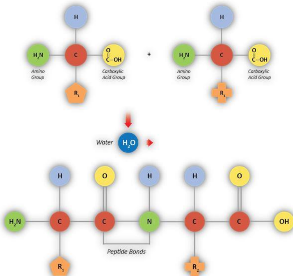
Figure 5: Formation of a peptide bond
