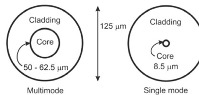
Figure 3.1 Optical Fiber Cross Sections
