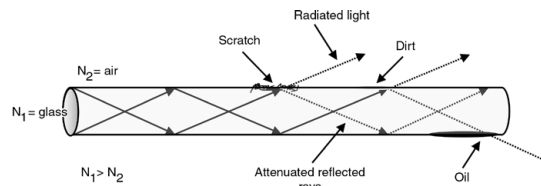
Figure 3.3 Problems Associated with a Glass Air Interface
