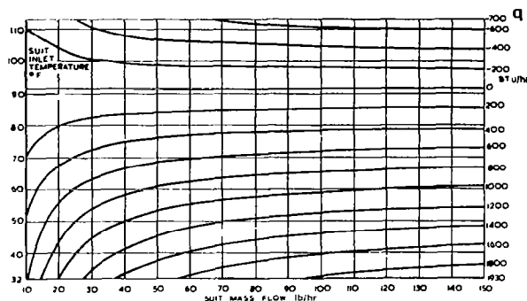
SUIT PERFORMANCE FOR AN EARLY PROTOTYPE LIQUID-COOLED SUIT
