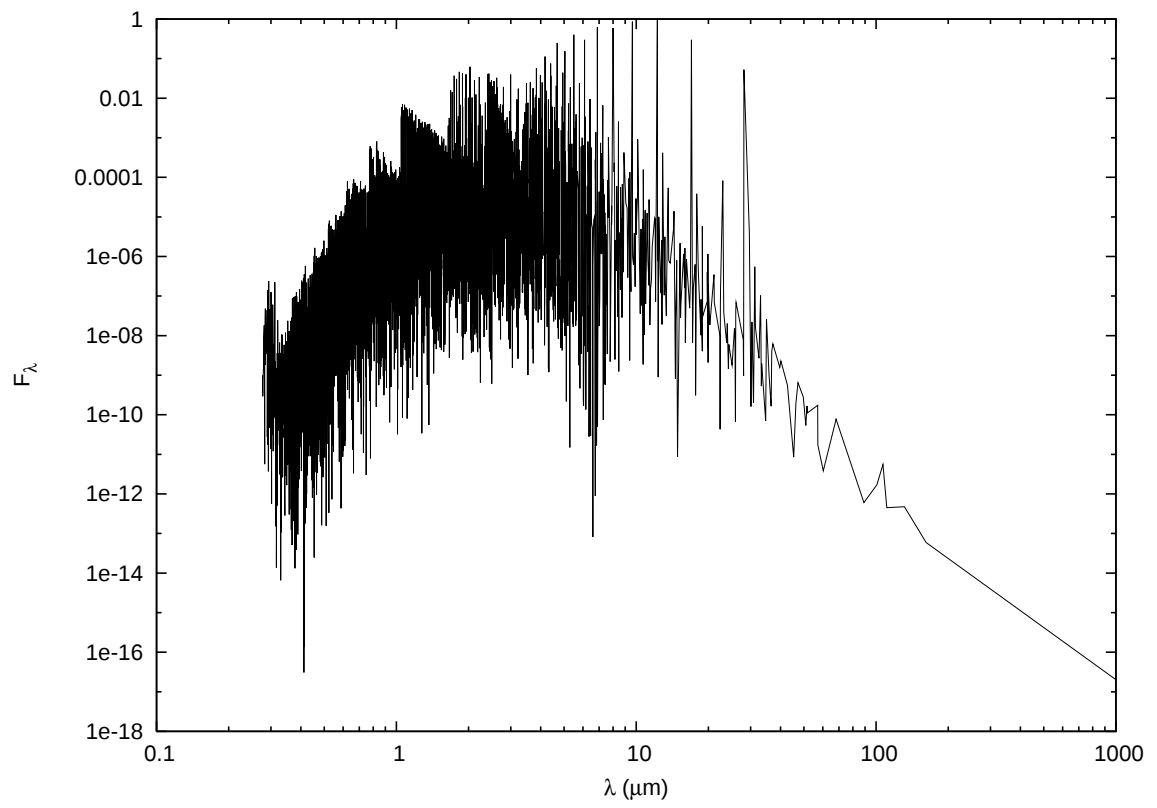
Figure 12 Mielke predicted spectrum T = 10000\text{K} n_H = 1\text{E}4\text{cm}^{-3}
