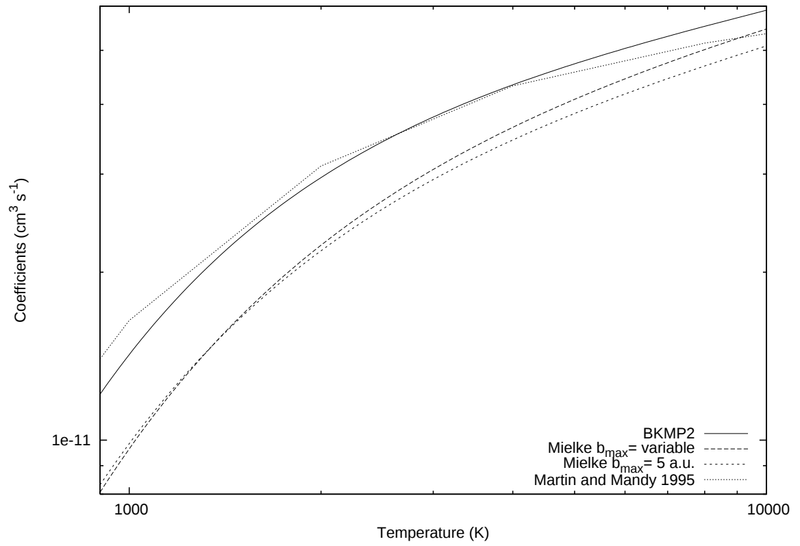
Figure 30 BKMP2 and Mielke coefficients for v=1,j=2 to v=1,j=0
