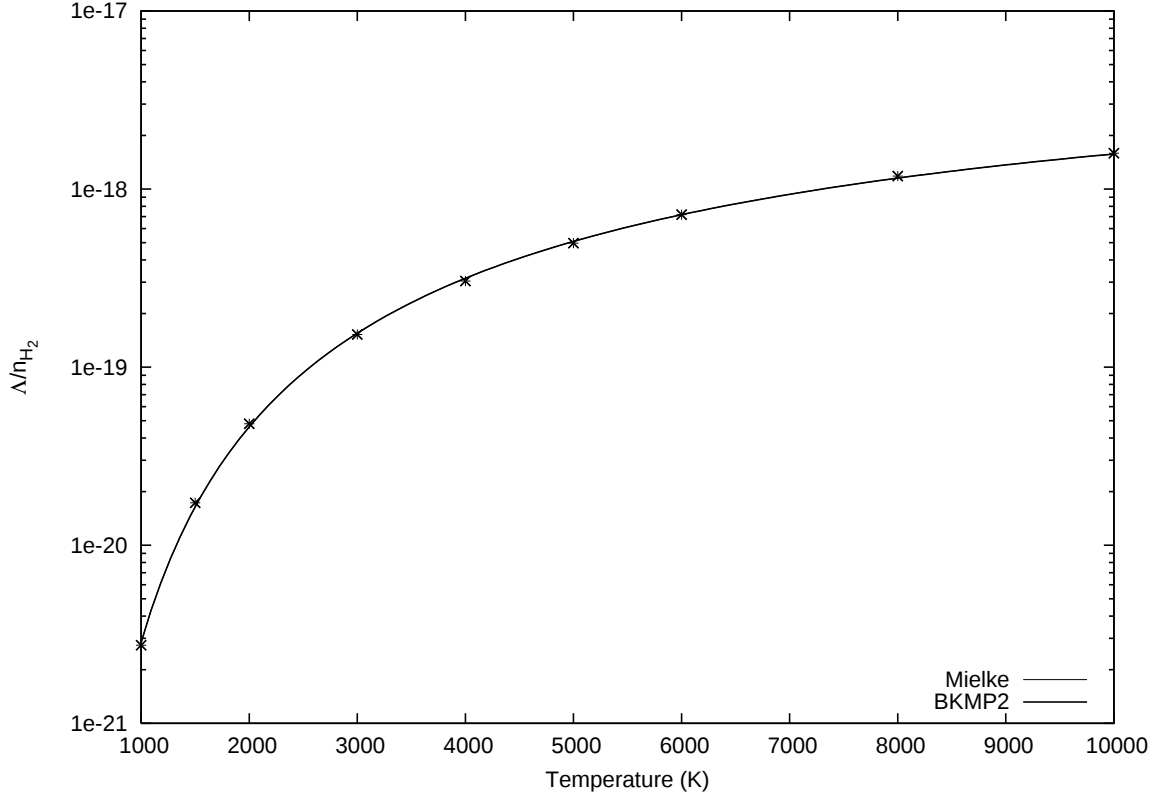
Figure 38 BKMP2 and Mielke cooling n_H = 1E8\text{cm}^{-3}
