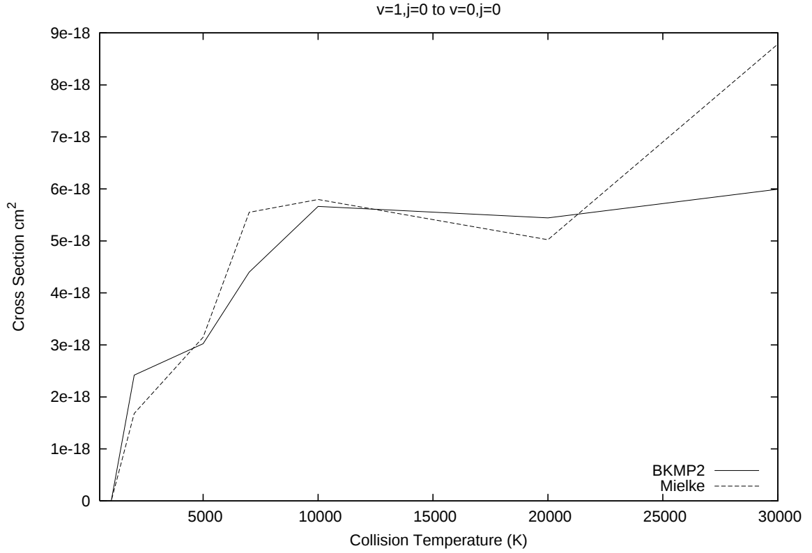
Figure 14 An example of a vibrational transition to a para state
