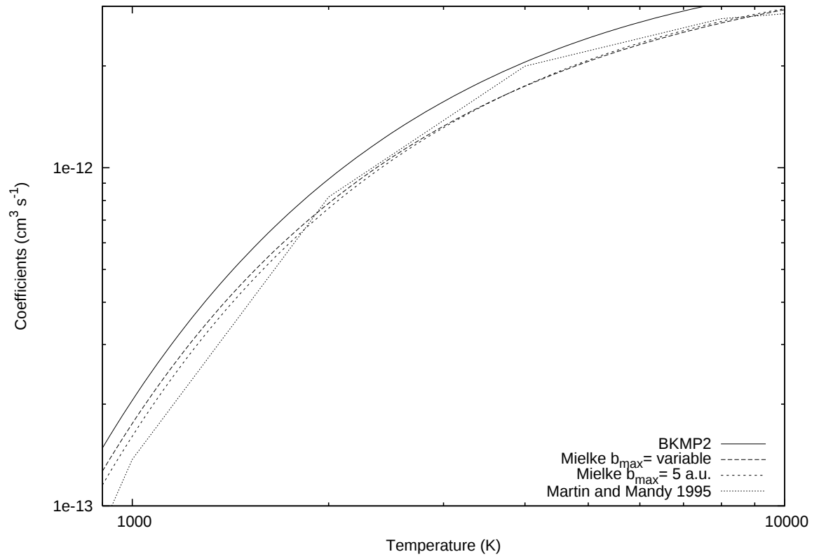
Figure 27 BKMP2 and Mielke coefficients for v=0, j=6 to v=0, j=0
