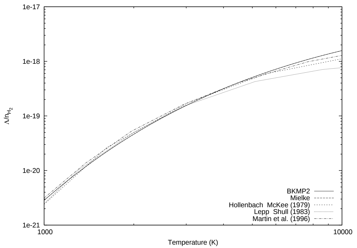
Figure 42 BKMP2 and Mielke with previous calculations n_H = 1\text{E}8\text{cm}^{-3}
