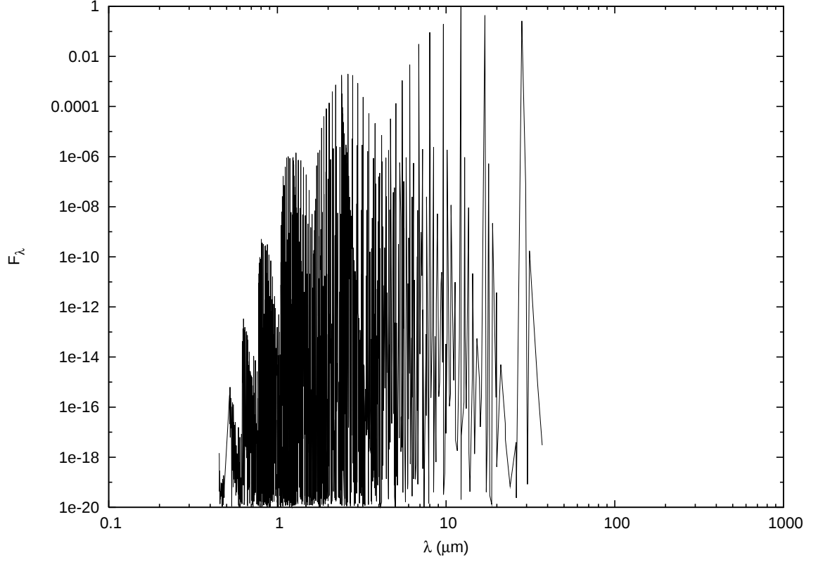
Figure 9 BKMP2 predicted spectrum T = 1000\text{K} n_H = 1\text{cm}^{-3}
