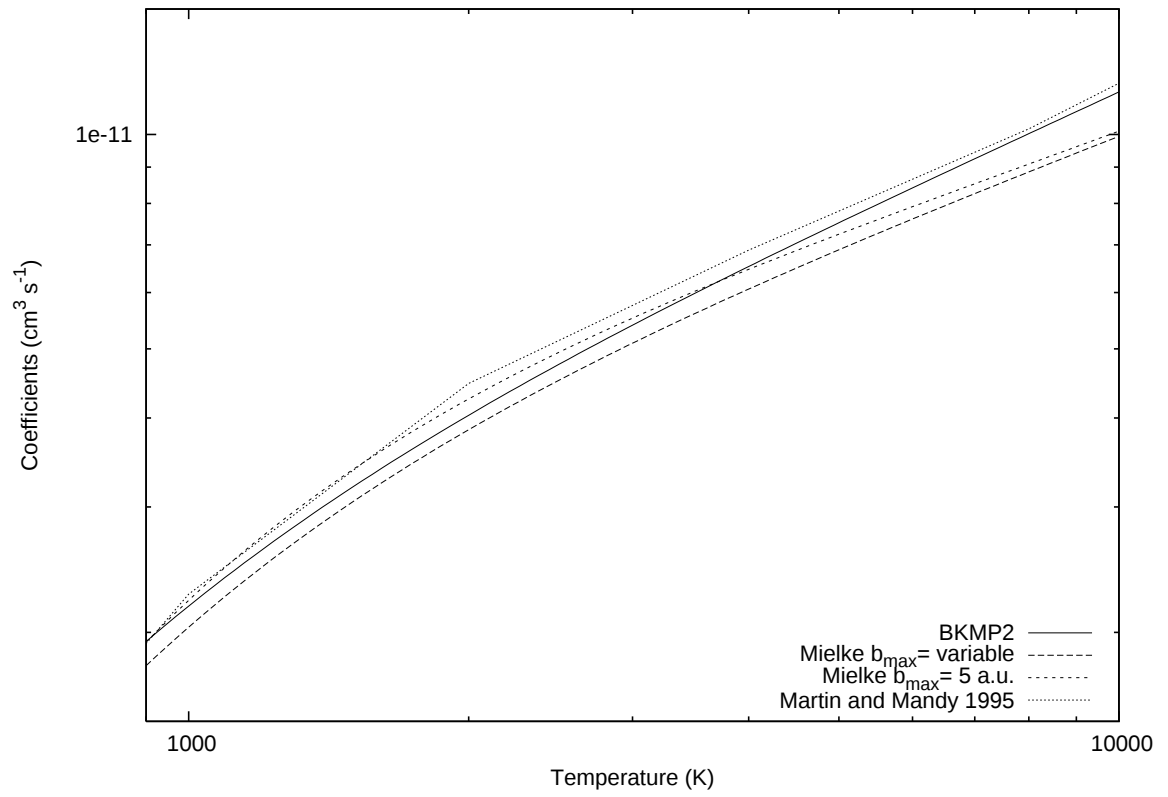
Figure 33 BKMP2 and Mielke coefficients for v=2,j=1 to v=0,j=1
