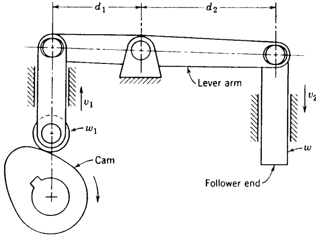
FIGURE 13.20. Lever ratio.
