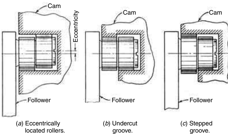
FIGURE 10.21. Roller and groove designs.
