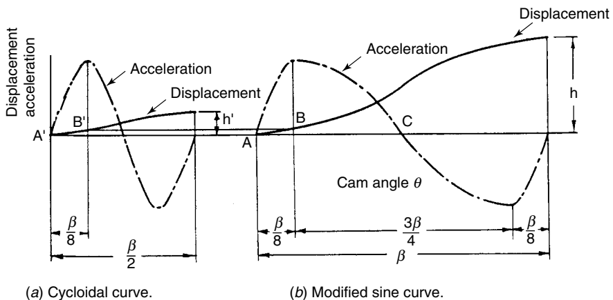
FIGURE 3.9. Modified sine curve.
