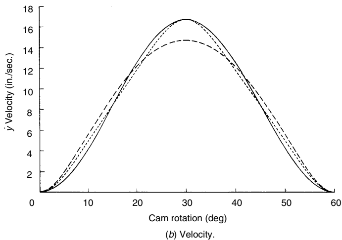
FIGURE 3.10. Comparison of popular curves (cam has 2-inch rise in 60-degree rotation and 3-inch pitch diameter). (Erdman and Sandor (1997) with permission by Prentice Hall, Upper Saddle River, N.J.)
