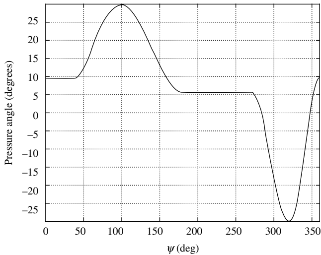
FIGURE 7.18. Pressure-angle distribution.
