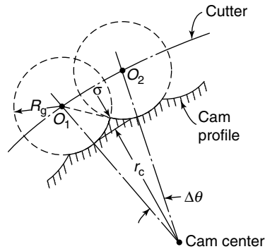
FIGURE 10.2. Increment cutting scallops.
