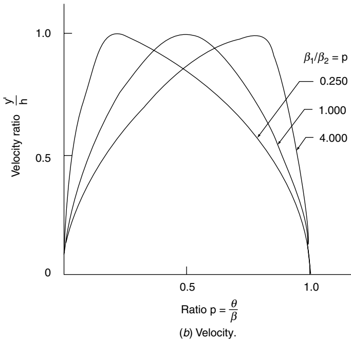
FIGURE 3.8. Skewed modified trapezoidal curve comparison (normalized h = 1 , \beta = 1 ).
