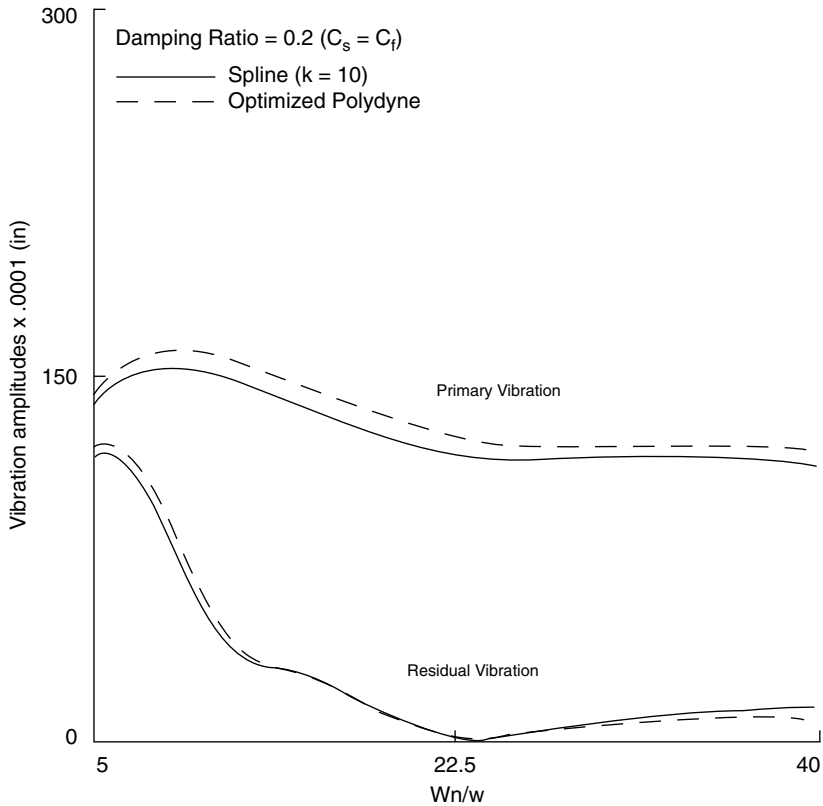
FIGURE 5.29. Amplitudes of primary and residual vibrations for both spline ( k = 10 ) optimized polydyne with damping ratio = 0.2 ( C_s = C_t ) in Example 8.
