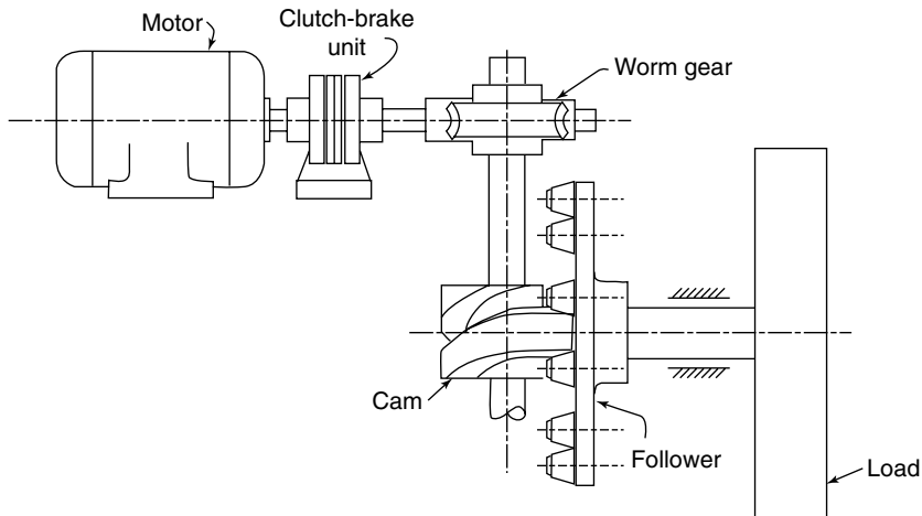
FIGURE 8.6. Cam indexing mechanism.
