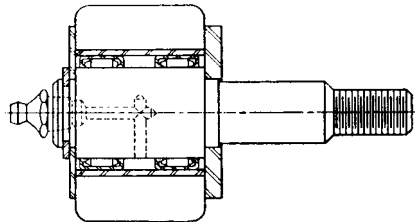
FIGURE 10.17. Roller follower constructed of standard needle bearings with laminated thermoset resin outer race.
