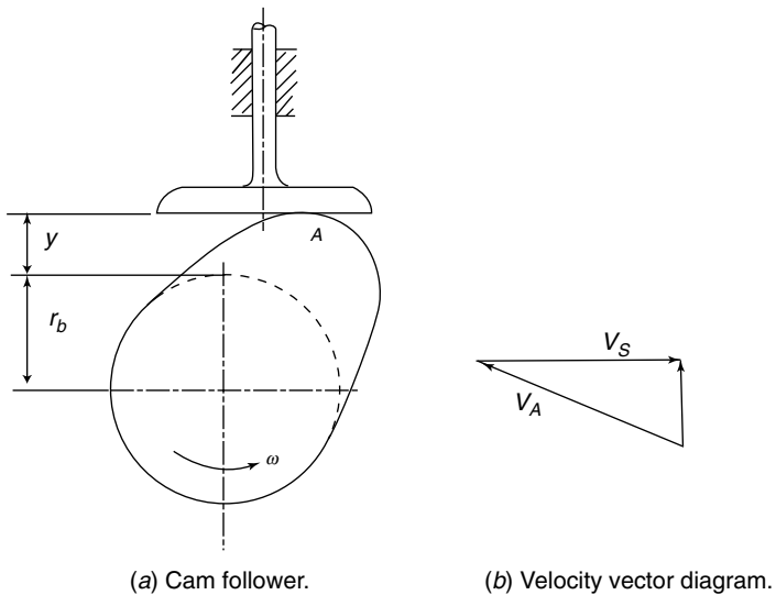
FIGURE 8.10. Cam and reciprocating flat-faced follower.
