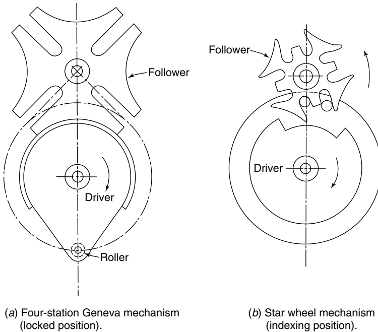
FIGURE 14.32. Some intermittent-motion mechanisms.
