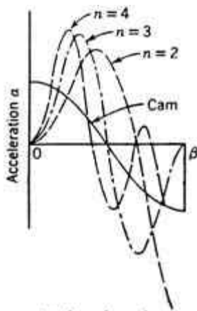
(c) Acceleration.
