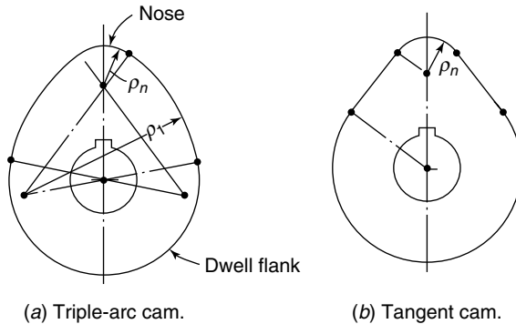
(a) Triple-arc cam. FIGURE 14.10. Circular arc cams.
