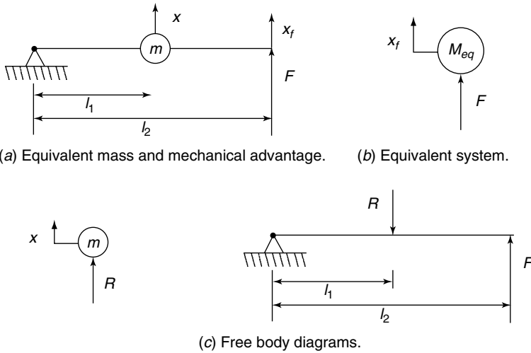
FIGURE 11.7. Equivalent mass and mechanical advantage.
