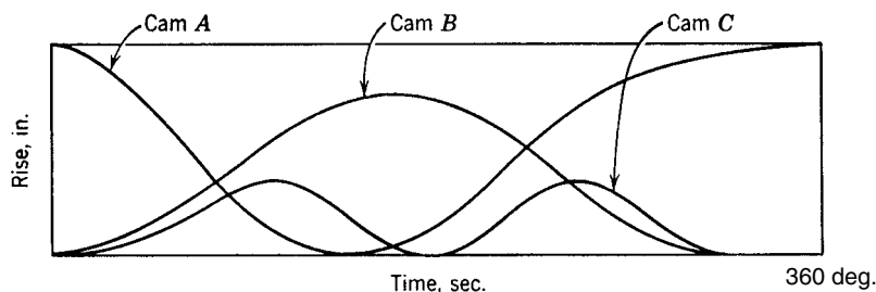
FIGURE 1.25. Time chart (showing compounding of three cams).
