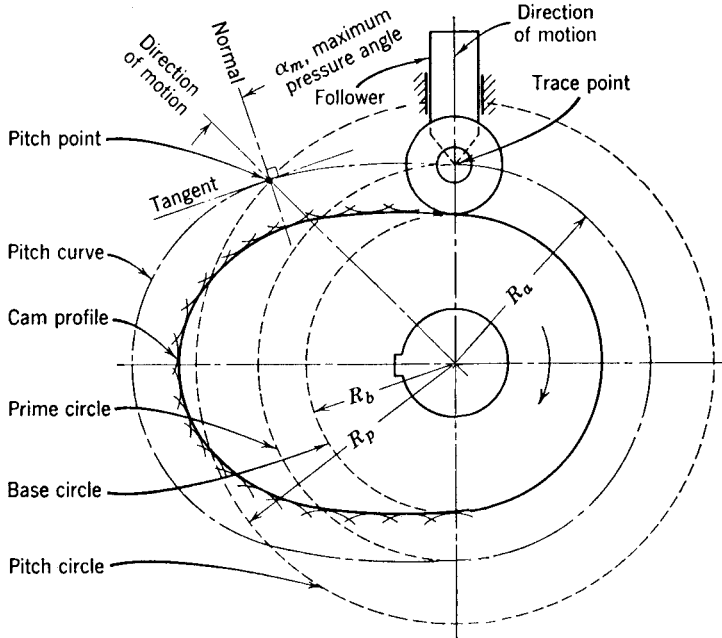
FIGURE 1.26. Cam nomenclature.
