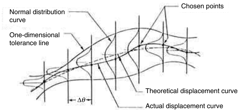
FIGURE 10.9. Combined effects of cam and follower tolerance on follower displacement curve.
