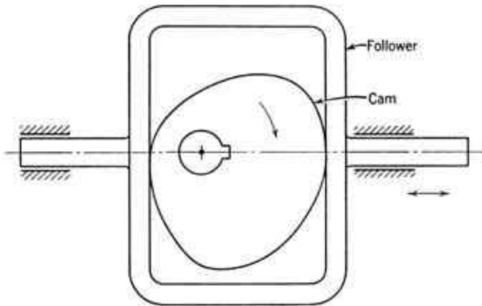
FIGURE 1.10. Yoke cam.
