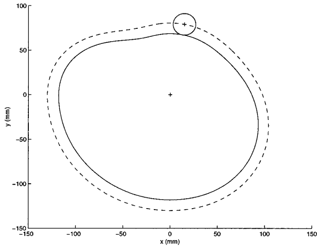
FIGURE 7.20. Pitch curve.
