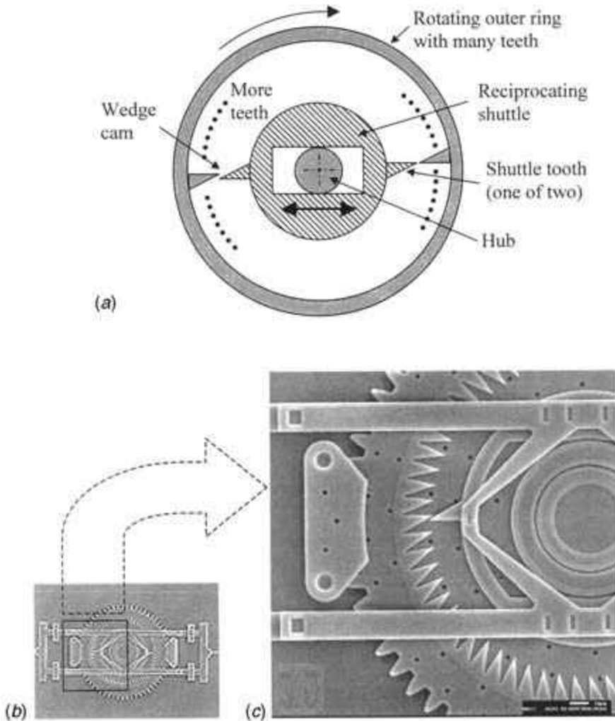
FIGURE 15.6. Indexing (wedge-cam) motor (a) schematic showing the principle of operation, (b) and (c) scanning electron microscope (SEM) picture of the microfabricated prototype (courtesy, Sandia National Labs—MEMS, S&T Department, www.mems.sandia.gov ).
