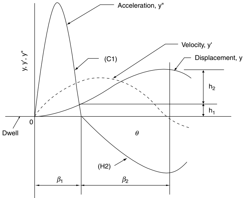
FIGURE 3.18. Cycloidal harmonic cam-follower motion example.
