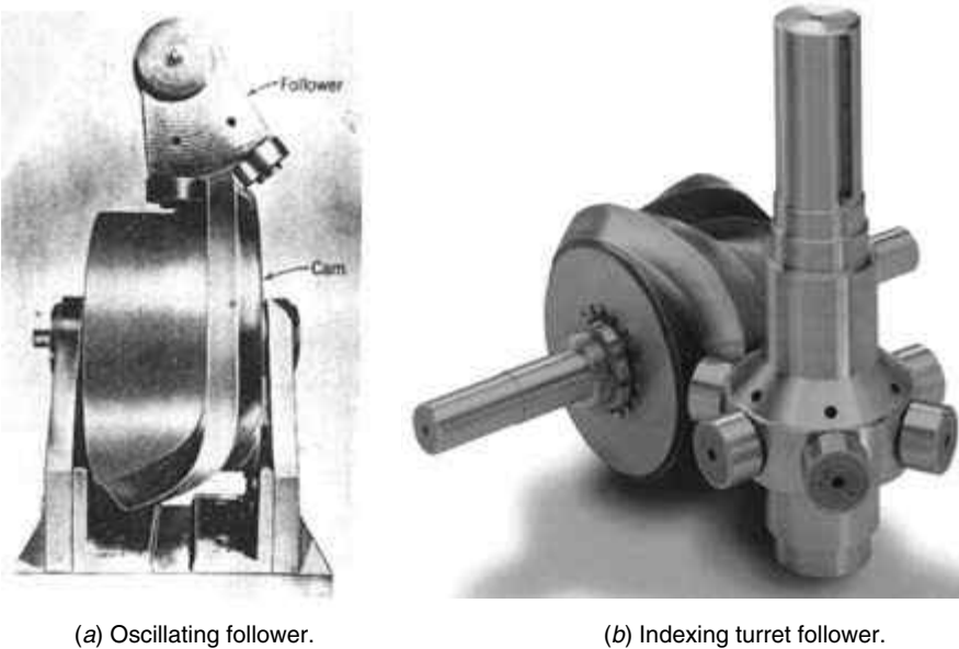
FIGURE 1.16. Globoidal cam-blade type (courtesy Ferguson Company St. Louis, Mo.).
