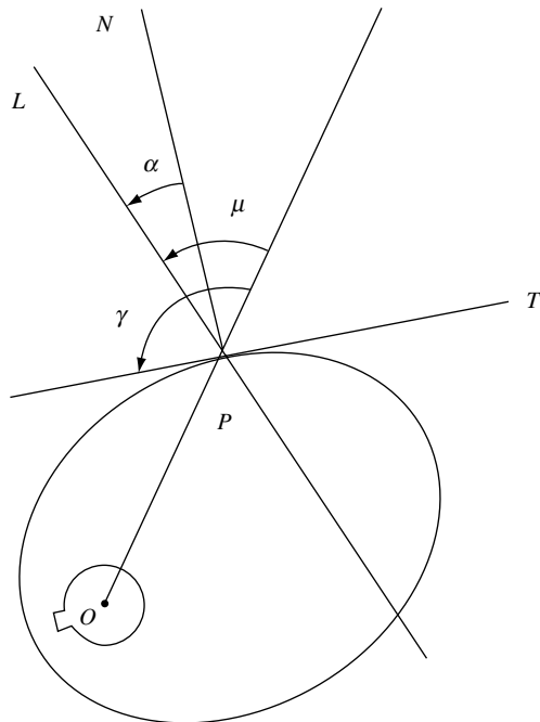
FIGURE 7.2. Notation for pressure-angle determination.
