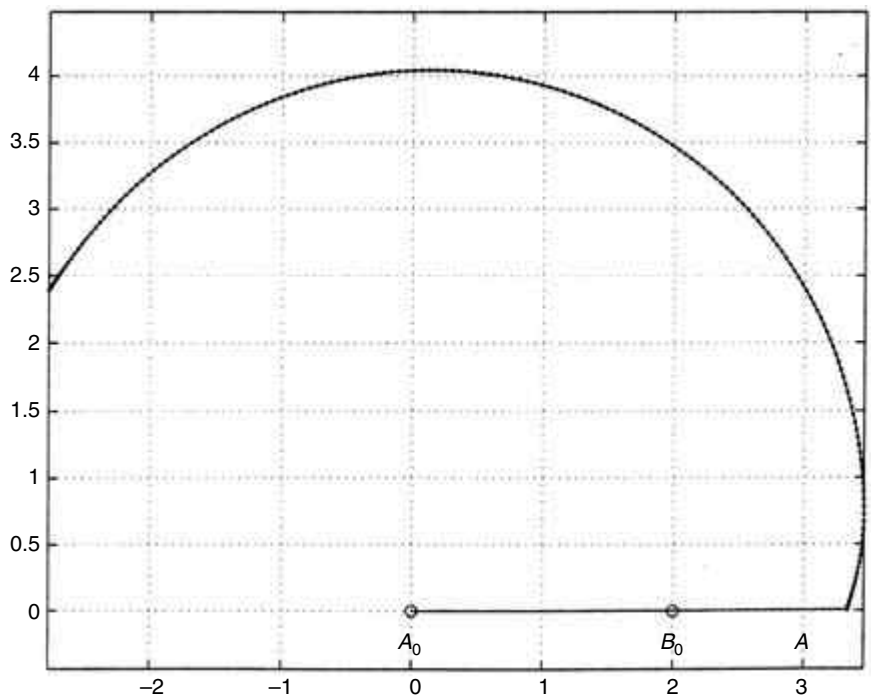
FIGURE 8.28. Cam profile obtained using the inversion technique for the single-dwell motion.
