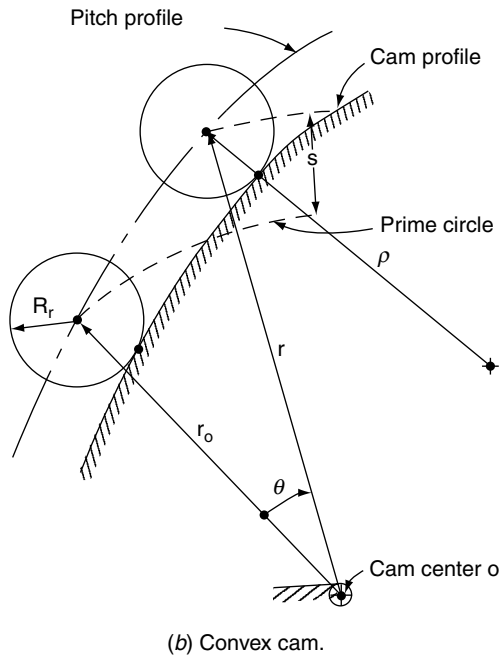
FIGURE 6.9 Typical cam contours.
