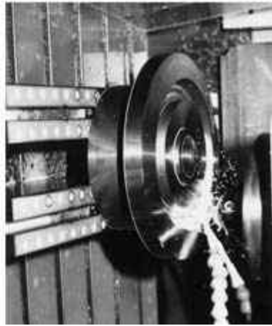
(c) Milling radial cam.
