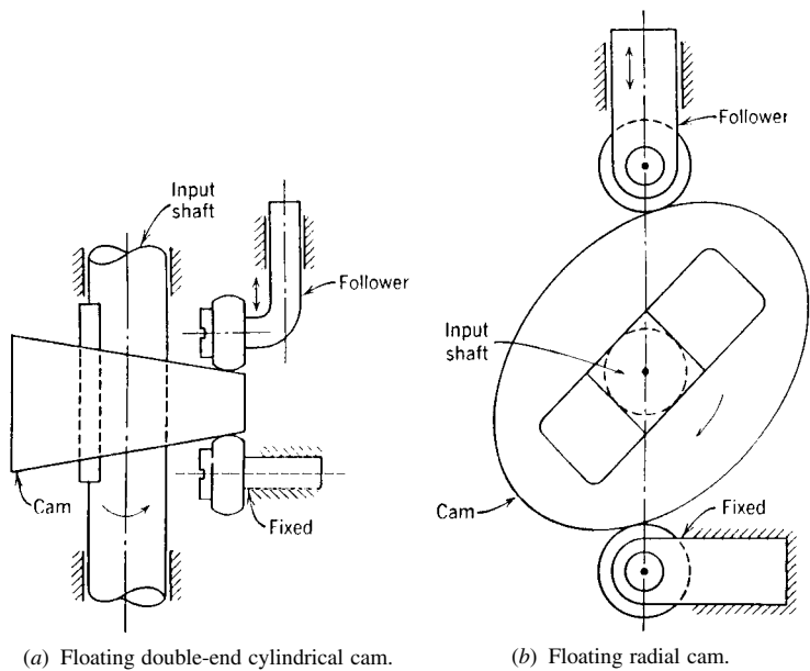
(a) Floating double-end cylindrical cam. (b) Floating radial cam. FIGURE 14.23. Increased stroke cams.
