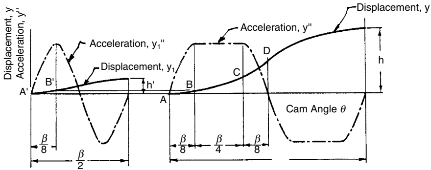
(a) Basic cycloidal curve.
