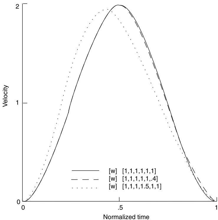
FIGURE 5.15. Comparison of cam-follower velocities in Example 5.
