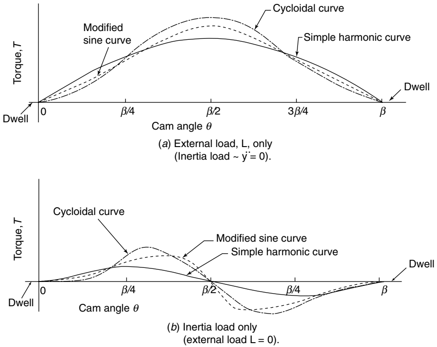
FIGURE 8.9. Torque comparison of cam curves (DRD cam).
