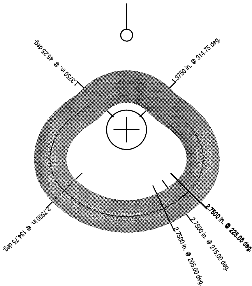
FIGURE E.7. B-12345 Sample cam plot of coordinate file.
