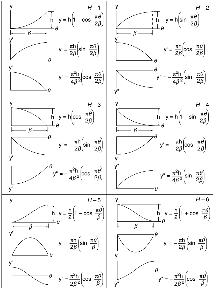
FIGURE 3.15. Harmonic motion characteristics.
