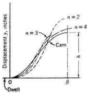
(a) Displacement.
