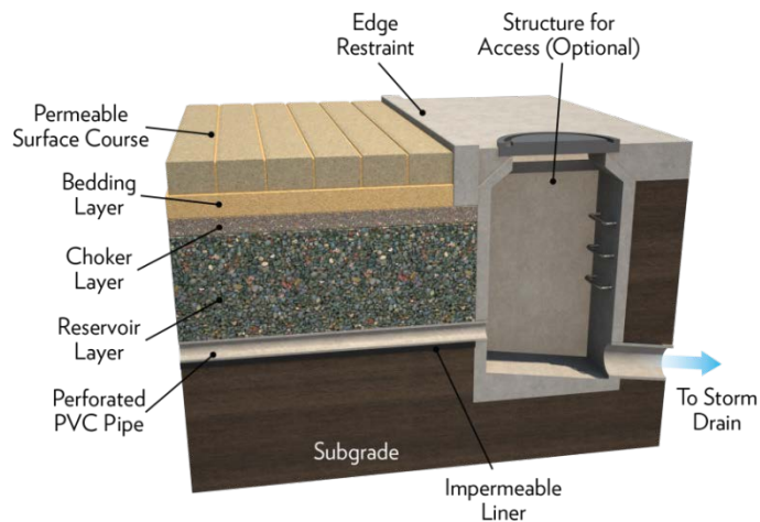
Reservoir layer with underdrain and impermeable liner
