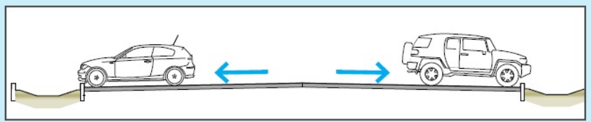
Crowned slope conveys half of each aisle to adjacent swale
