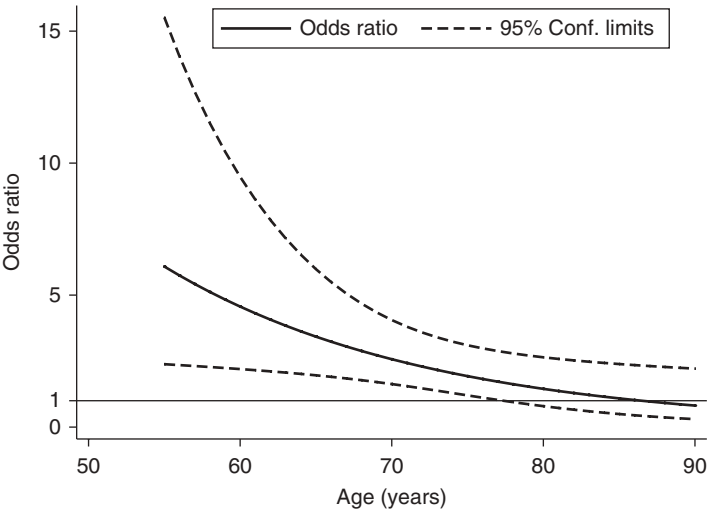
Figure 3.5 Plot of the estimated odds ratio for PRIORFRAC = 1 versus PRIORFRAC = 0 as a function of age, with 95% confidence bands.
