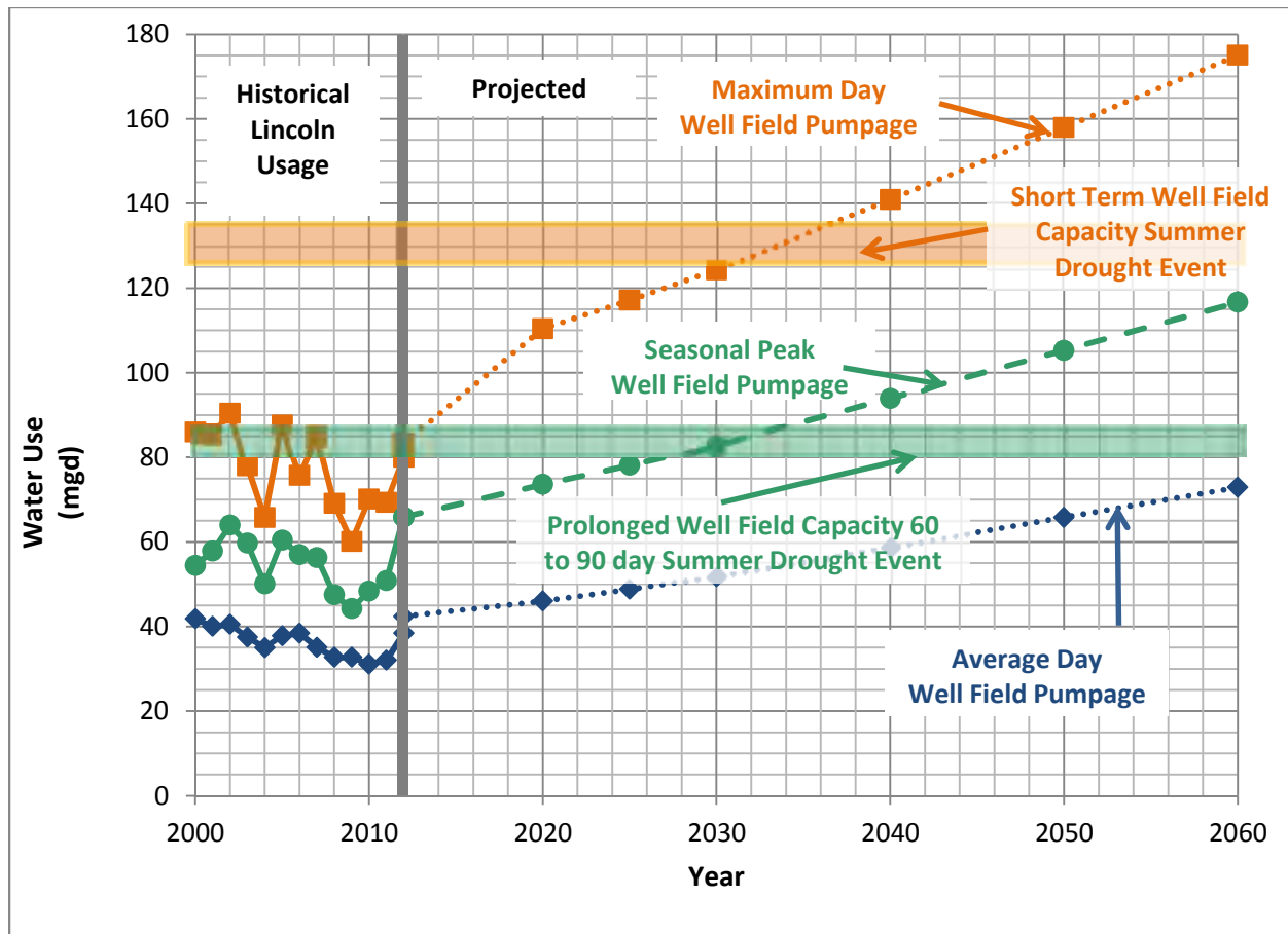
Figure 4-1 Raw Water Supply with the Fourth HCW and Revised Deficits over Planning Horizon
