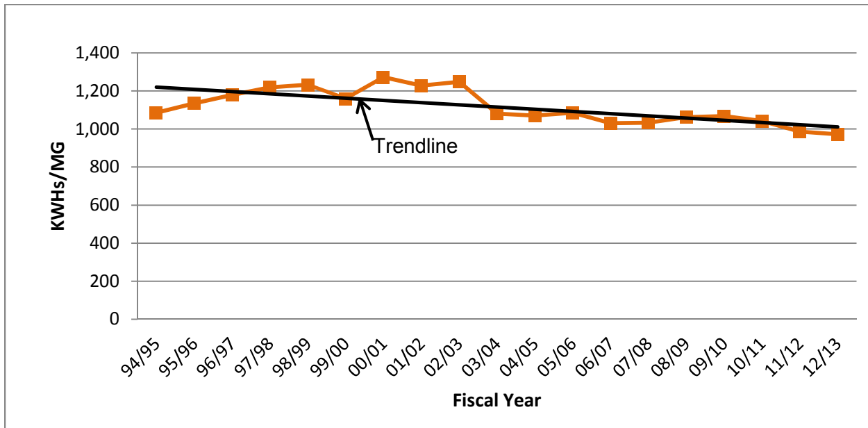
Figure 2-6 Energy Usage in KWHs/Million Gallons per Fiscal Year
