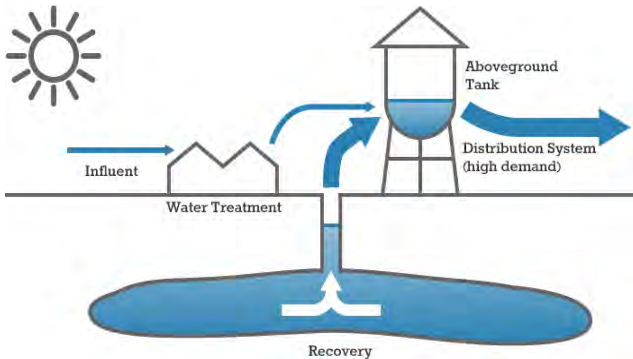
Figure 4-6 ASR Recovery Cycle
