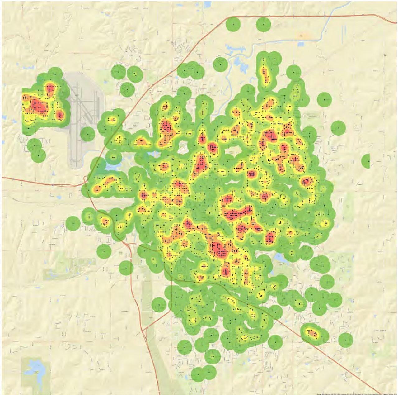
Figure 3-2 Main Break Density
