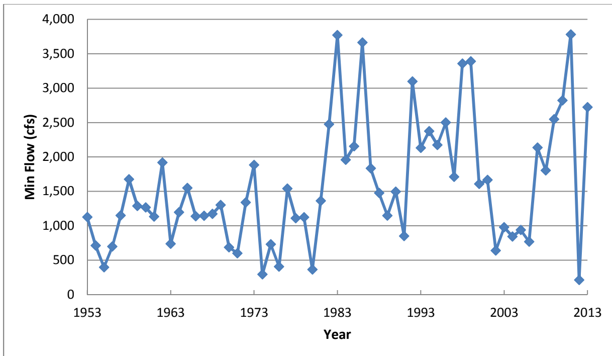
Figure 2-14 30-day Minimum Flow for USGS Gage at North Bend
