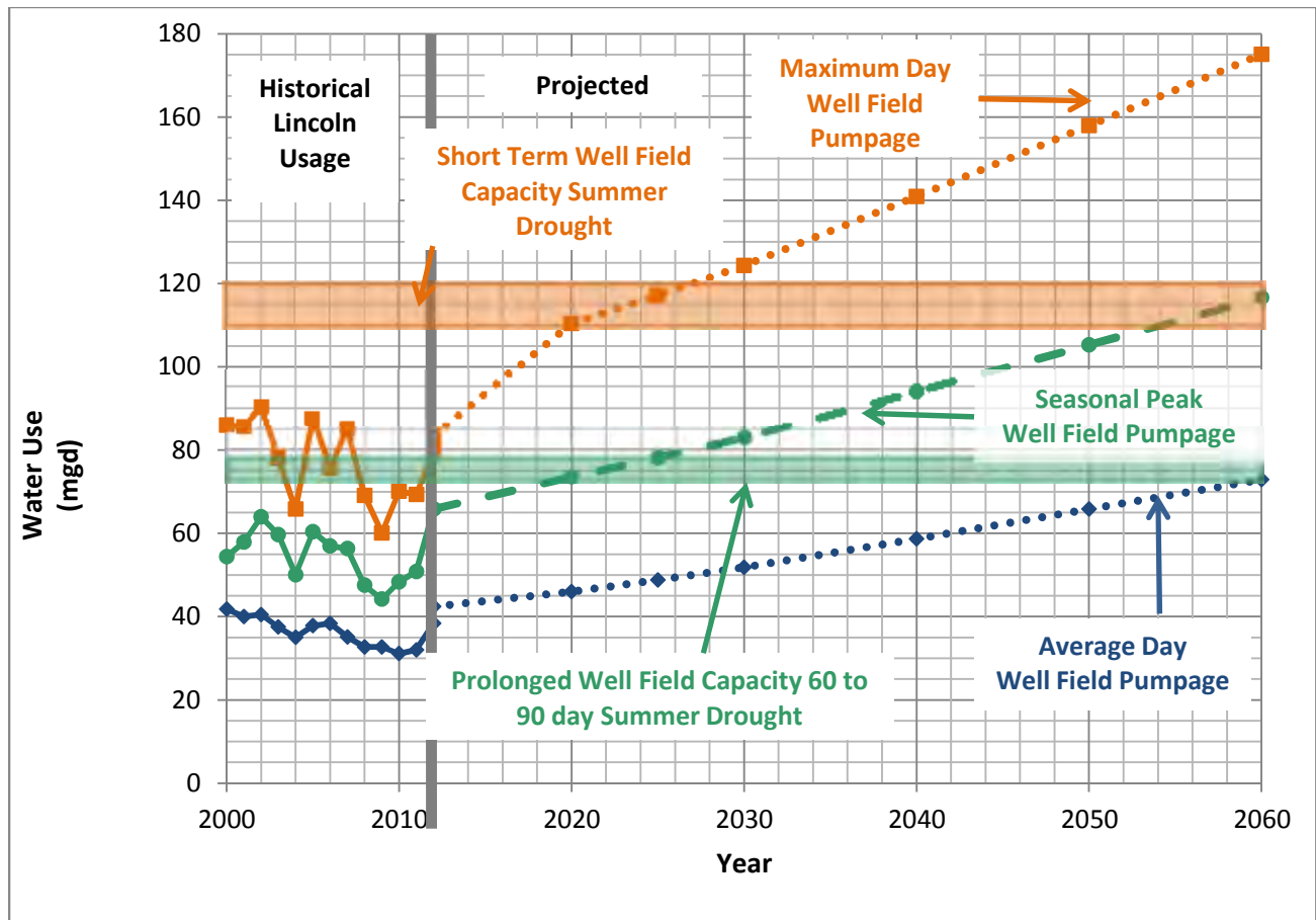
Figure 3-4 Raw Water Supply Deficits over Planning Horizon (with the Third HCW)
