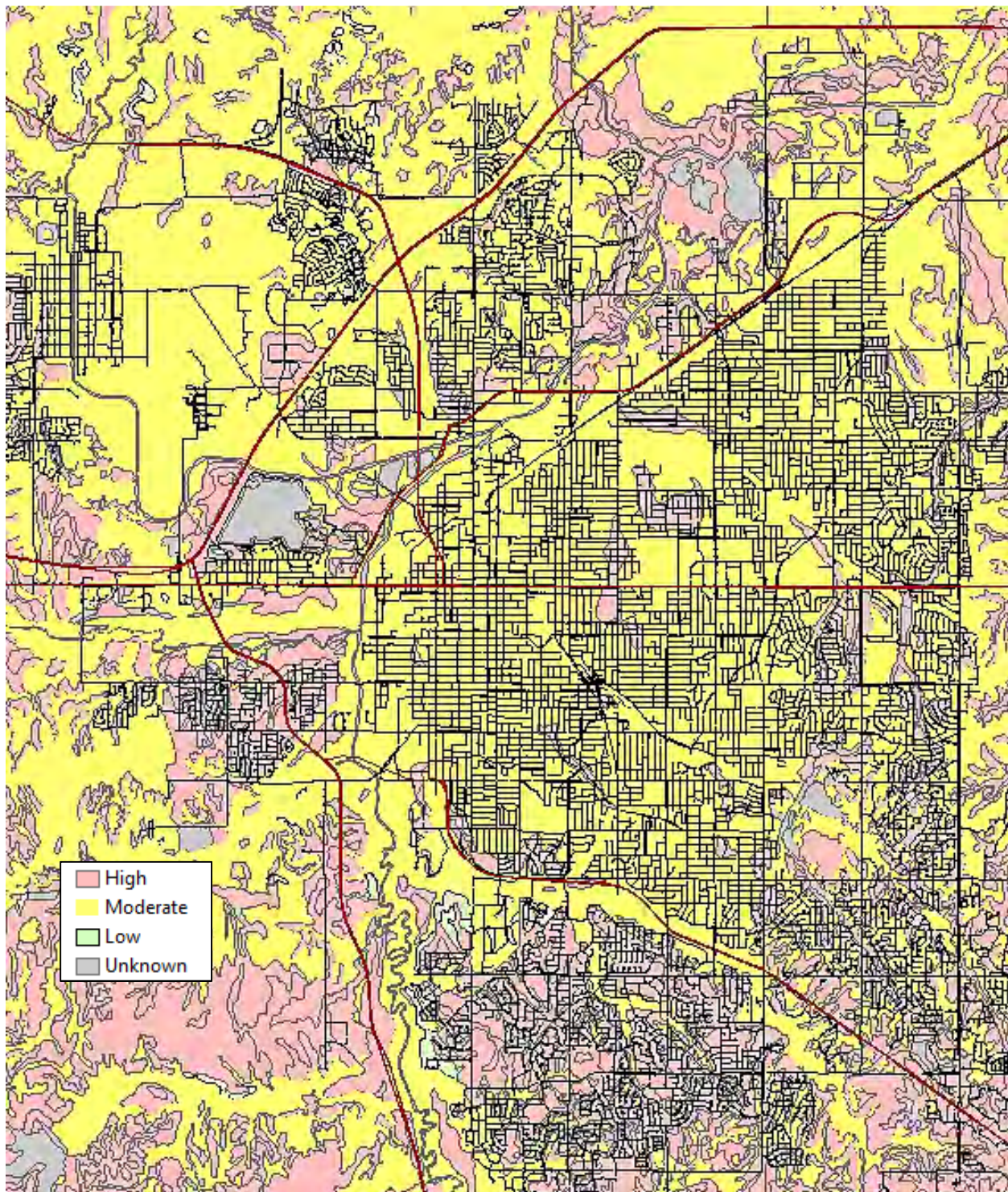
Figure 3-17 Soil Corrosion Potential Map
