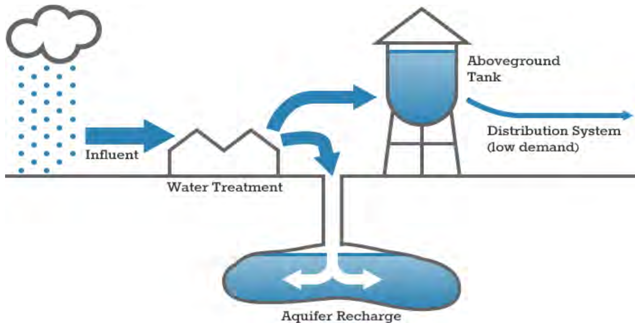
Figure 4-5 ASR Injection Cycle
