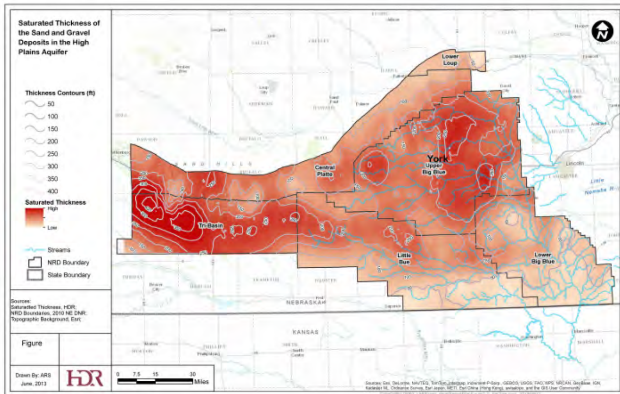
Figure 4-2 Saturated Thickness of High Plains Aquifer West of Lincoln
