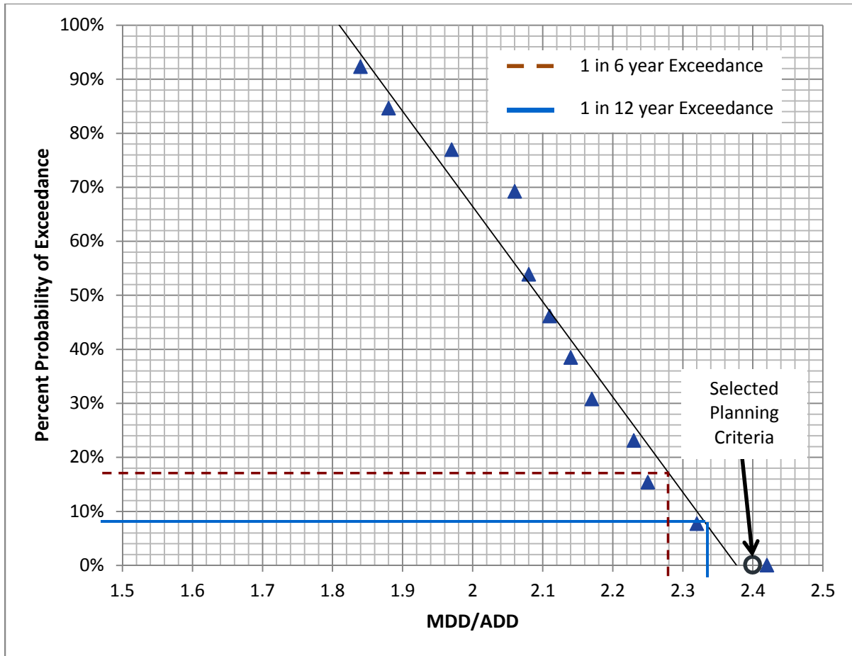
Figure 3-6 MDD:ADD, Percent Probability of Exceedance
