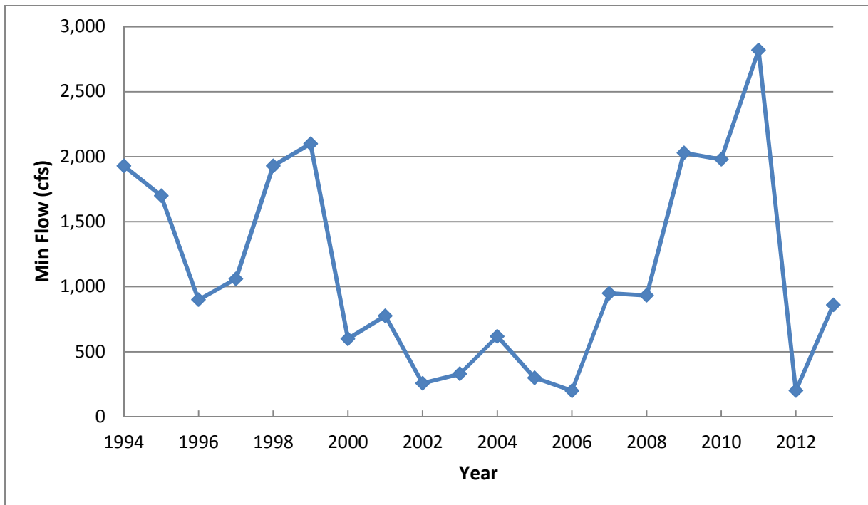
Figure 2-15 1-day Minimum Flow for USGS Gage near Leshara
