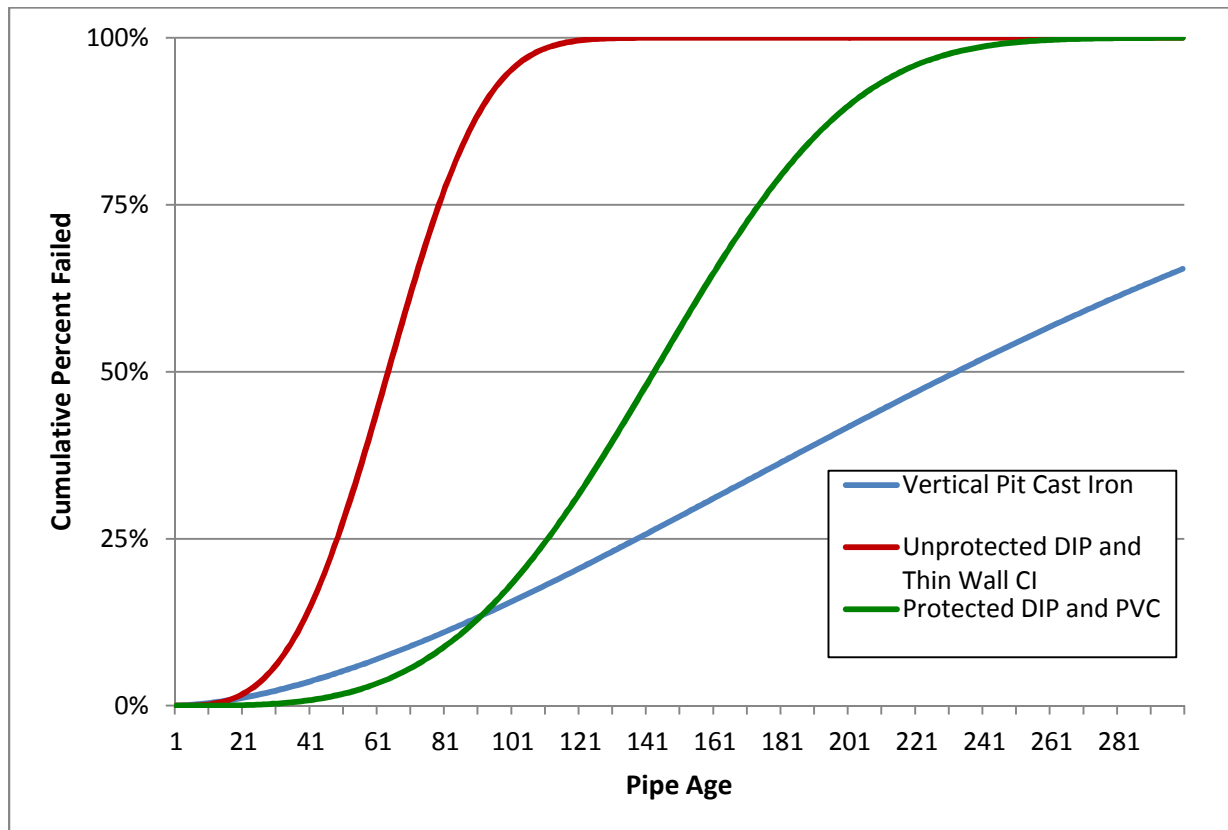
Figure 4-3 Weibull Cumulative Distribution Function
