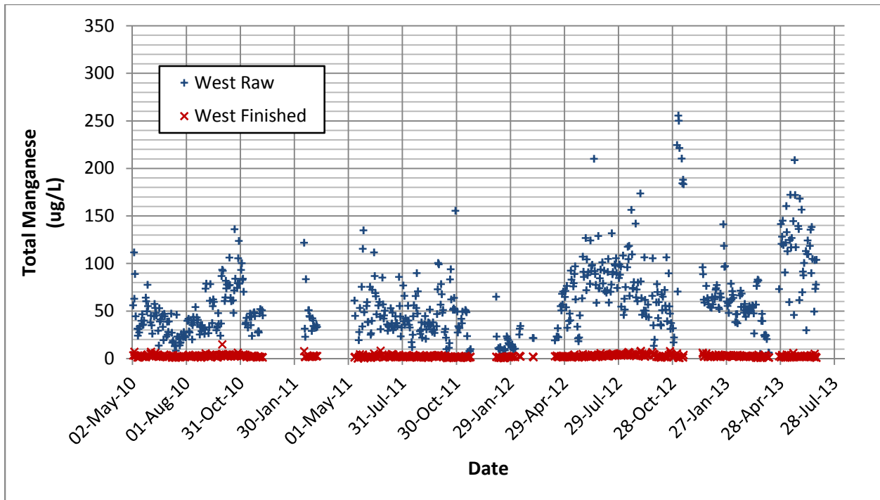
Figure 3-2 West Plant Total Manganese
