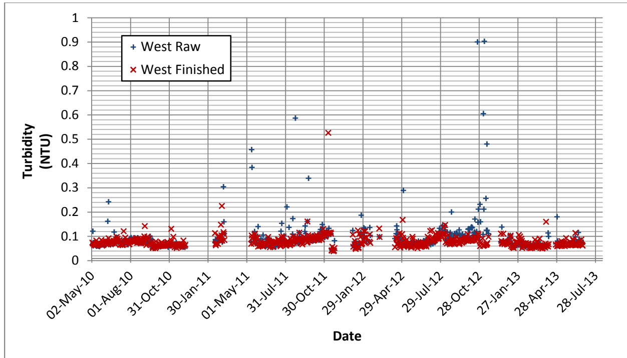
Figure 3-4 West Plant Turbidity
