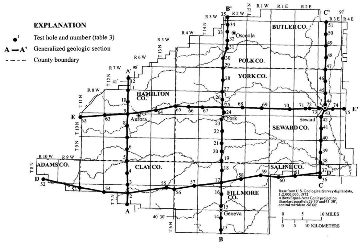
Figure 3. Locations of test holes and generalized geologic sections (figure 4).
