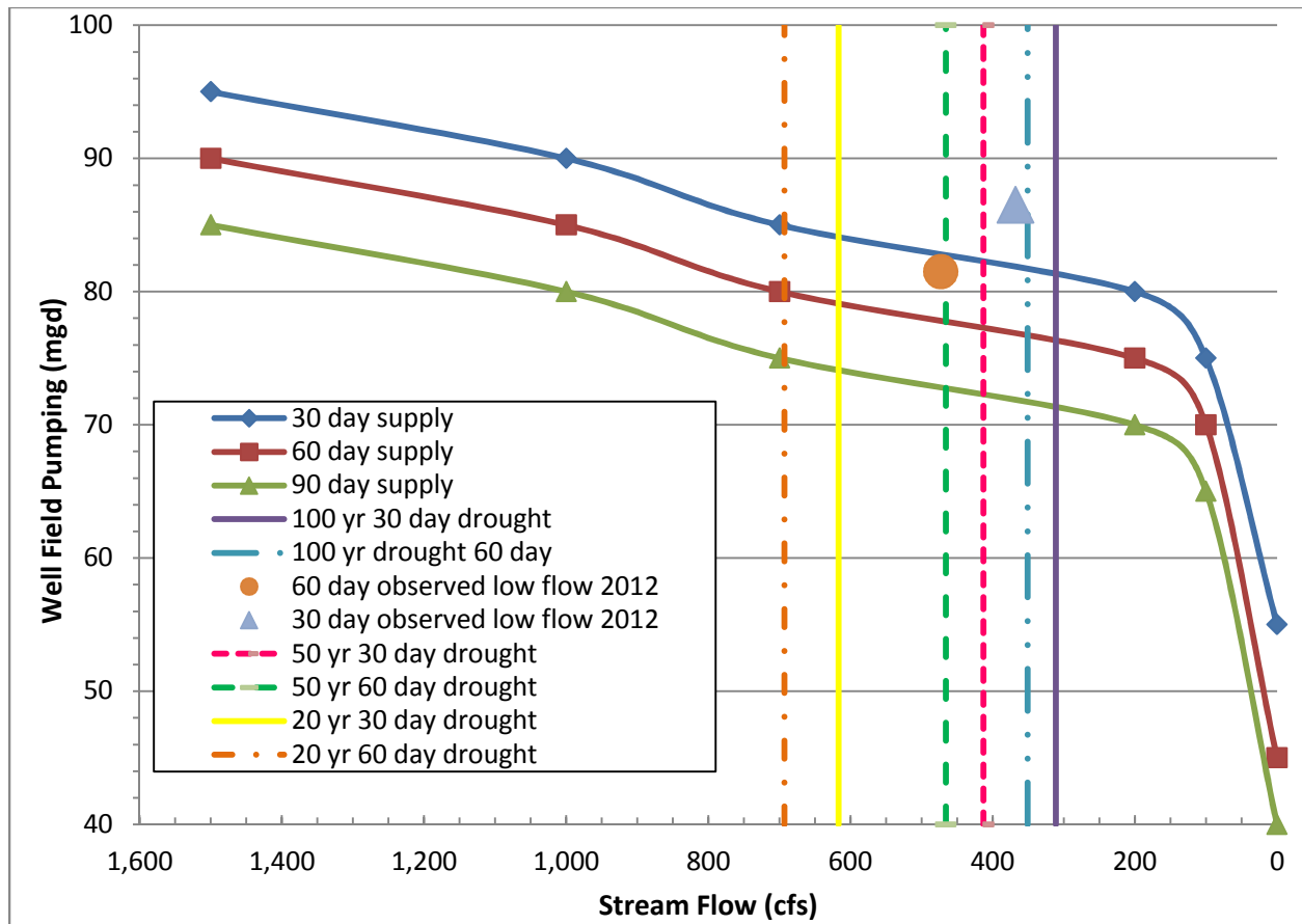
Figure 3-3 Model-Predicted Well Field Capacity with third HCW and Drought Reoccurrence Interval Window
