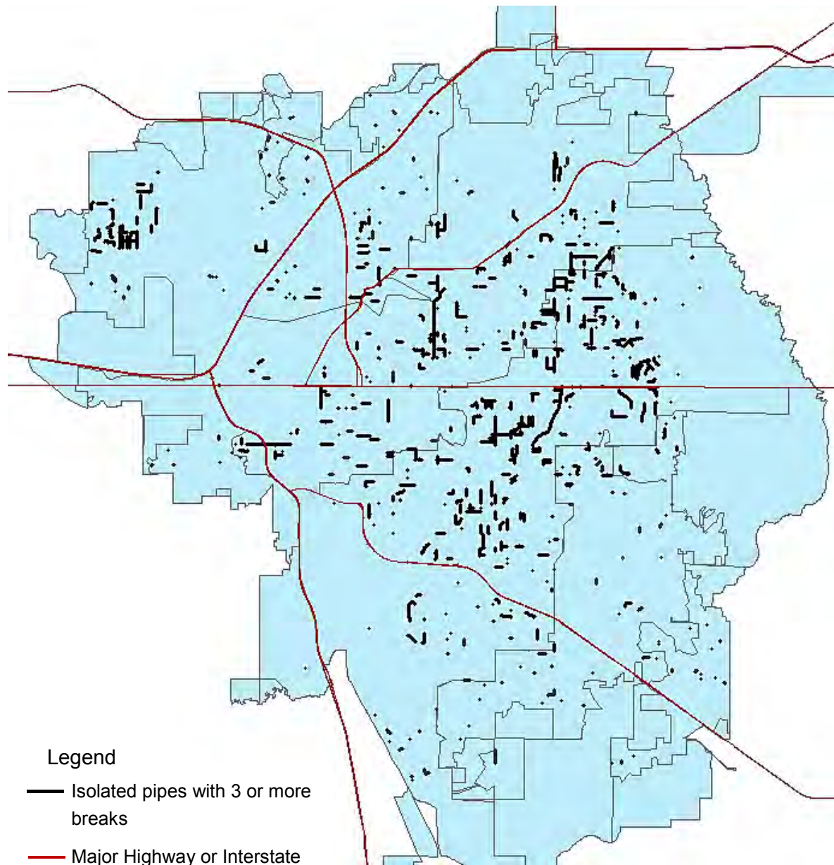
Figure 4-2 Pipe Network Map
