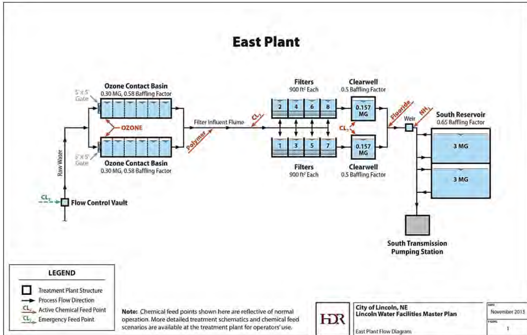
Figure 2-1 East Plant Process Flow Diagram
