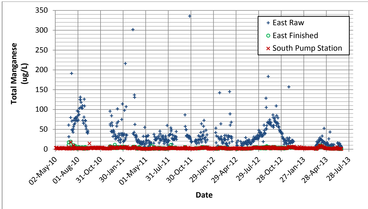
Figure 3-1 East Plant Total Manganese
