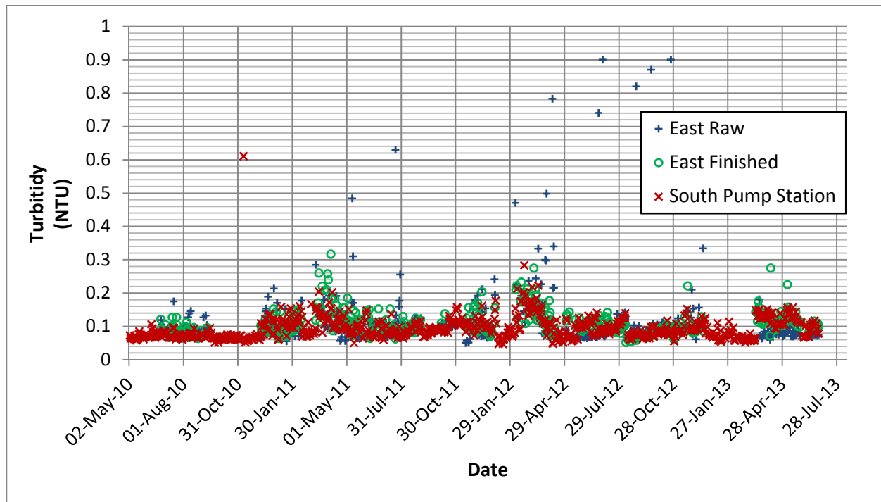
Figure 3-3 East Plant Turbidity
