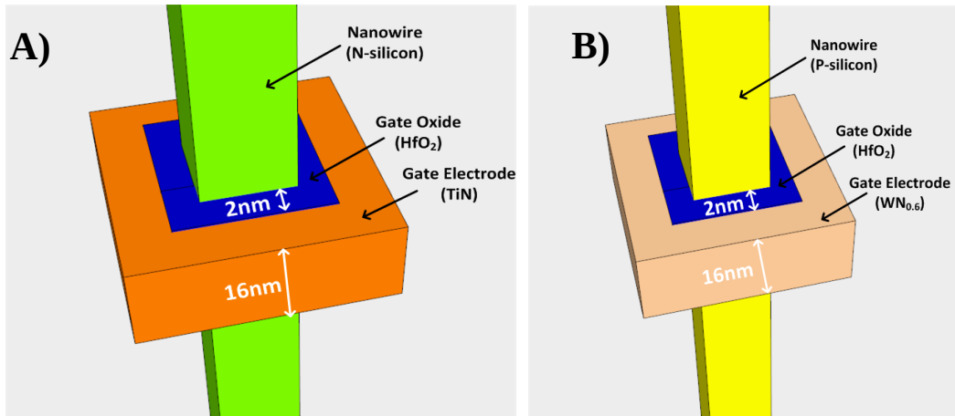
Figure.3.3 Vertical GAA junctionless transistors: A) n-type transistor with gate material TiN and B) p-type transistor with gate material WN 0.6
