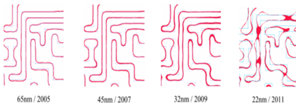
Figure. 1.4 Lithographic challenges with scaling [4]
