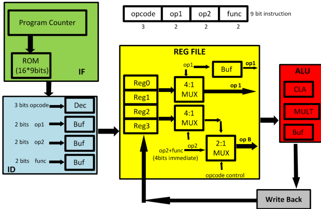
Figure.7.6Architecture Block Diagram
