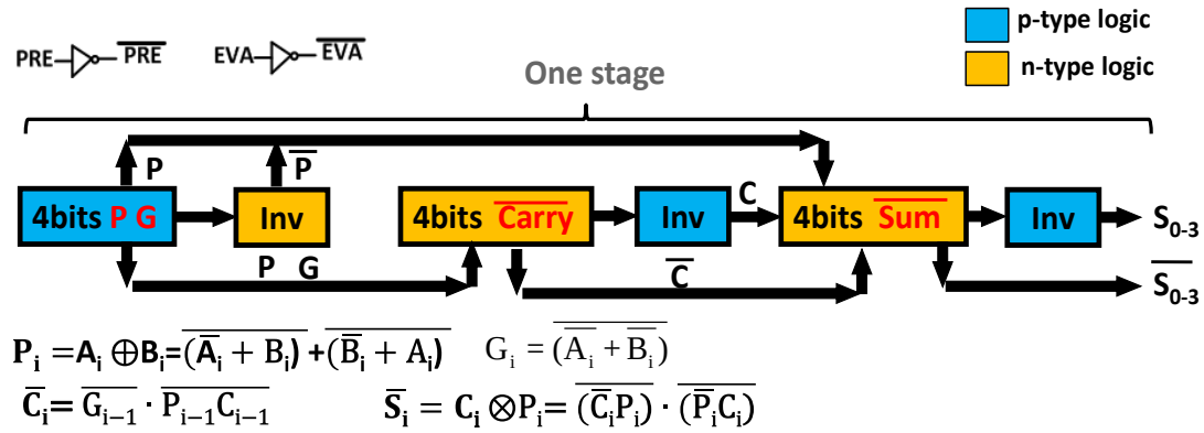
Figure.5.1 Block diagram of 4-bit CLA
