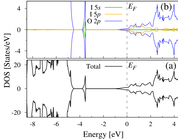
Figure 2.6: Calculated TDOS (a) and PDOS (b) plots for I-doped \text{SnO}_2 .
