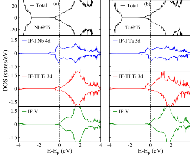
Figure 3.3: Calculated spin-polarized total and partial DOS projected on Ti 3d, Nb 4d, and Ta 5d orbitals near the interfacial region of the STO substrate for (a) Nb@Ti and (b) Ta@Ti doped LAO/STO HS systems. The IF-I, IF-III, and IF-V represent the first, third and fifth layers in the STO substrate, respectively. The Fermi level is indicated by the vertical dashed line at 0 eV.
