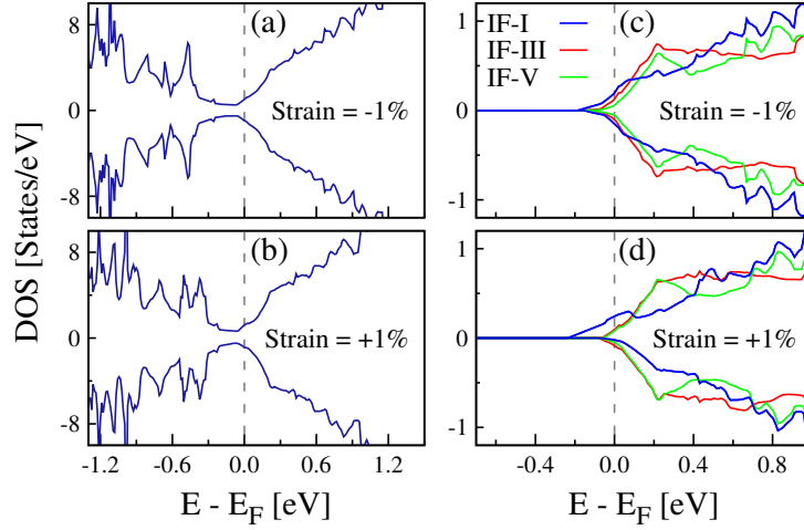
Figure 4.4: Calculated spin-polarized total DOS for n -type (\text{LAO})_5/\text{STO} HS slab systems under -1% (a) and +1% (b) [100] uniaxial strain. Calculated partial DOS of Ti 3d orbitals from IF-I, IF-III, and IF-V TiO 2 layers in the STO substrate of the same systems under -1% (c) and +1% (d) [100] uniaxial strain.
