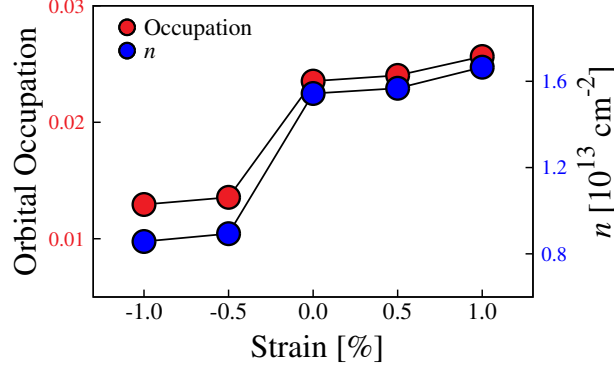
Figure 4.5: Calculated orbital occupation numbers and respective charge carrier densities ( n ) of Ti 3d orbitals at the interfacial TiO 2 layer in the STO substrate with respect to [100] uniaxial strain in the (LAO) 5 /STO HS slab systems.
