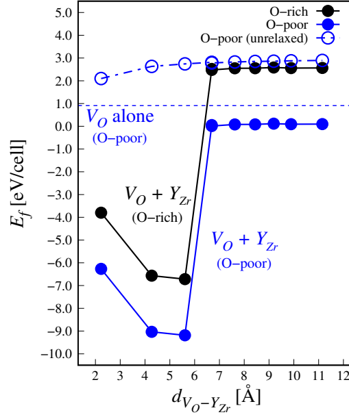
Figure 6.8: System formation energy in bulk Y-doped cubic \text{ZrO}_2 with respect to the distance between oxygen vacancy and substitutional Y ( d_{V_O-Y_{Zr}} ) under oxygen-rich (black) and oxygen-poor (blue) conditions. The blue horizontal dashed line indicates the oxygen vacancy formation energy in a pristine 324-atom supercell of cubic \text{ZrO}_2 .
