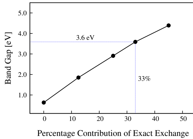
Figure 2.1: Dependence of calculated \text{SnO}_2 band gap on the percent contribution of exact Hartree-Fock (HF) exchange. The dashed blue line indicates HF percentage at which the experimental band gap is reproduced.
