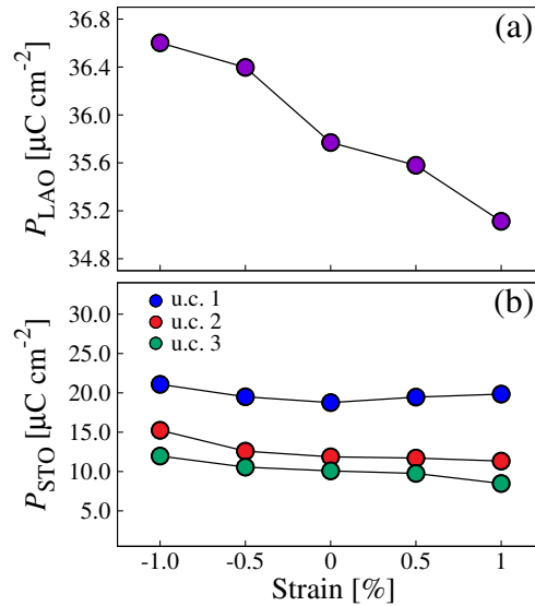
Figure 4.3: Calculated average polarization ( P_{\text{LAO}} ) in the LAO film (a), and in the first (blue), second (red), and third (green) STO unit cells (b) with respect to [100] uniaxial strain from -1\% to +1\% on the STO substrate in (\text{LAO})_5/\text{STO} HS slab systems.
