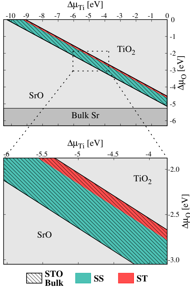
Figure 5.2: Grain boundary (GB) energy phase diagram with respect to \Delta\mu_{Ti} and \Delta\mu_O for the possible \text{SrTiO}_3 \Sigma 5 [001] twist GB structures. The striped area indicates the region of bulk \text{SrTiO}_3 stability. The turquoise and red areas indicate the energetically favored regions for the S/S and S/T GB models, respectively.
