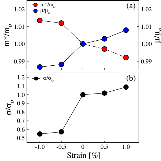
Figure 4.7: (a) Calculated normalized electron effective masses ( m^*/m_o ) and corresponding mobilities ( \mu/\mu_o ), and (b) normalized electrical conductivities ( \sigma/\sigma_o ) for Ti 3d electrons in the interfacial TiO 2 layer with respect to [100] uniaxial strain in (LAO) 5 /STO HS slab systems.
