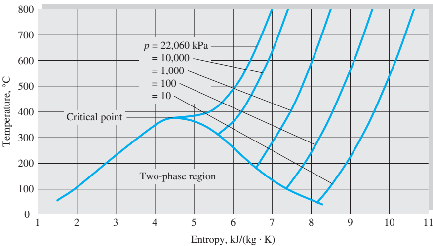
Fig. 1.3 Temperature-entropy chart for steam. The critical point is p_c = 22,060 \text{ kPa} , T_c = 374^\circ\text{C} , S_c = 4.41 \text{ kJ}/(\text{kg} \cdot \text{K}) . Except near the critical point, the smooth isobars tempt one to assume, often incorrectly, that the ideal-gas law is valid for steam. It is not , except at low pressure and high temperature: the upper right of the graph.
