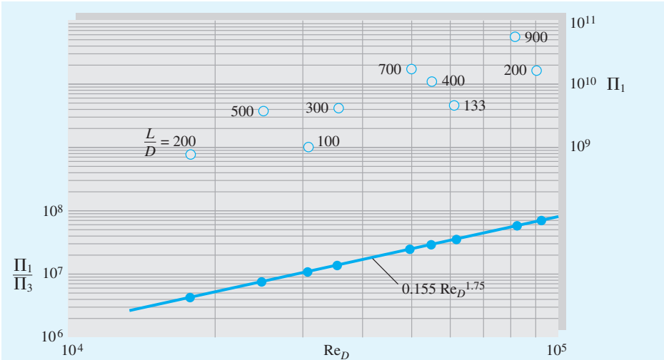
Fig. 5.10 Two different correlations of the data in Example 5.10: Open circles when plotting \rho D^2 \Delta p/\mu^2 versus Re_D , L/D is a parameter; once it is known that \Delta p is proportional to L , a replot (solid circles) of \rho D^3 \Delta p/(L\mu^2) versus Re_D collapses into a single power-law curve.
