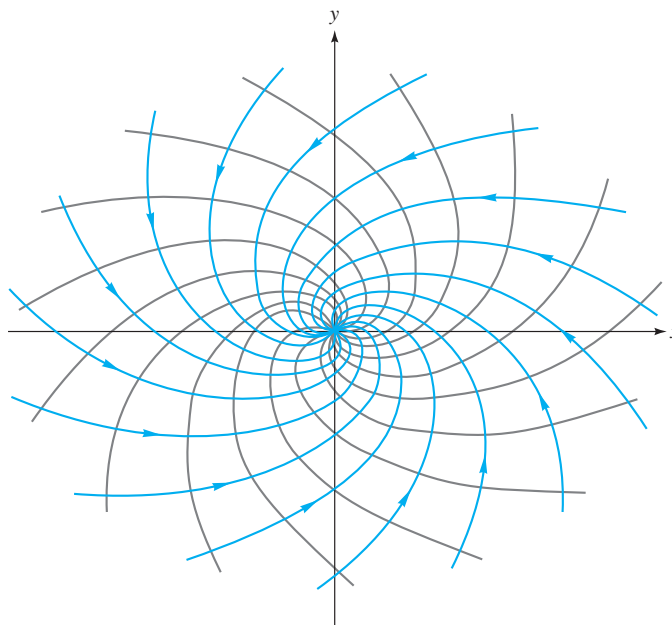
Fig. 8.5 Superposition of a sink plus a vortex, Eq. (8.16), simulates a tornado.
