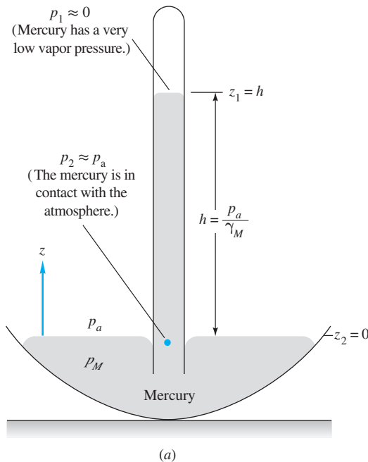
Fig. 2.6 A barometer measures local absolute atmospheric pressure: (a) the height of a mercury column is proportional to p_{\text{atm}} ; (b) a modern portable barometer, with digital readout, uses the resonating silicon element of Fig. 2.28c. (Courtesy of Paul Lupke, Druck, Inc.)
