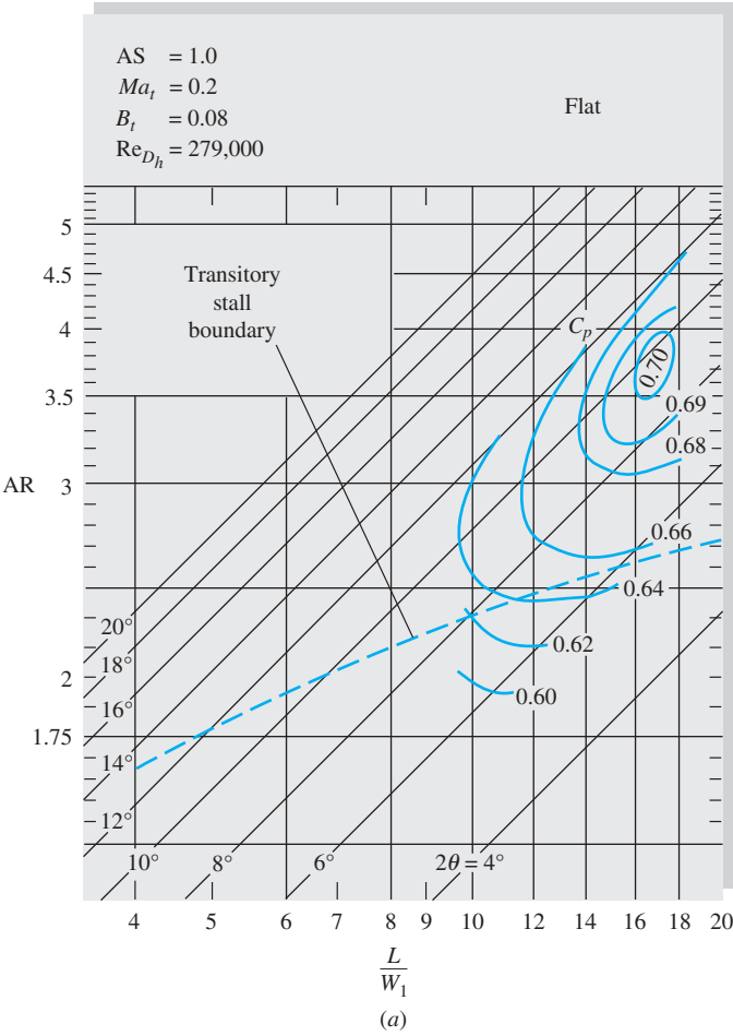
Fig. 6.28a Typical performance maps for flat-wall and conical diffusers at similar operating conditions: flat wall. Source: From P. W. Runstadler, Jr., et al., “Diffuser Data Book,” Crème Inc. Tech. Note 186, Hanover, NH, 1975., by permission of Creare, Inc.
