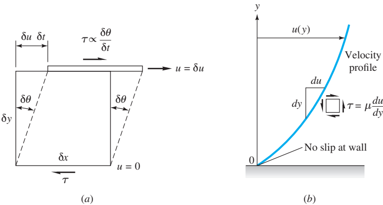
Fig. 1.5 Shear stress causes continuous shear deformation in a fluid: (a) a fluid element straining at a rate \delta\theta/\delta t ; (b) newtonian shear distribution in a shear layer near a wall.
