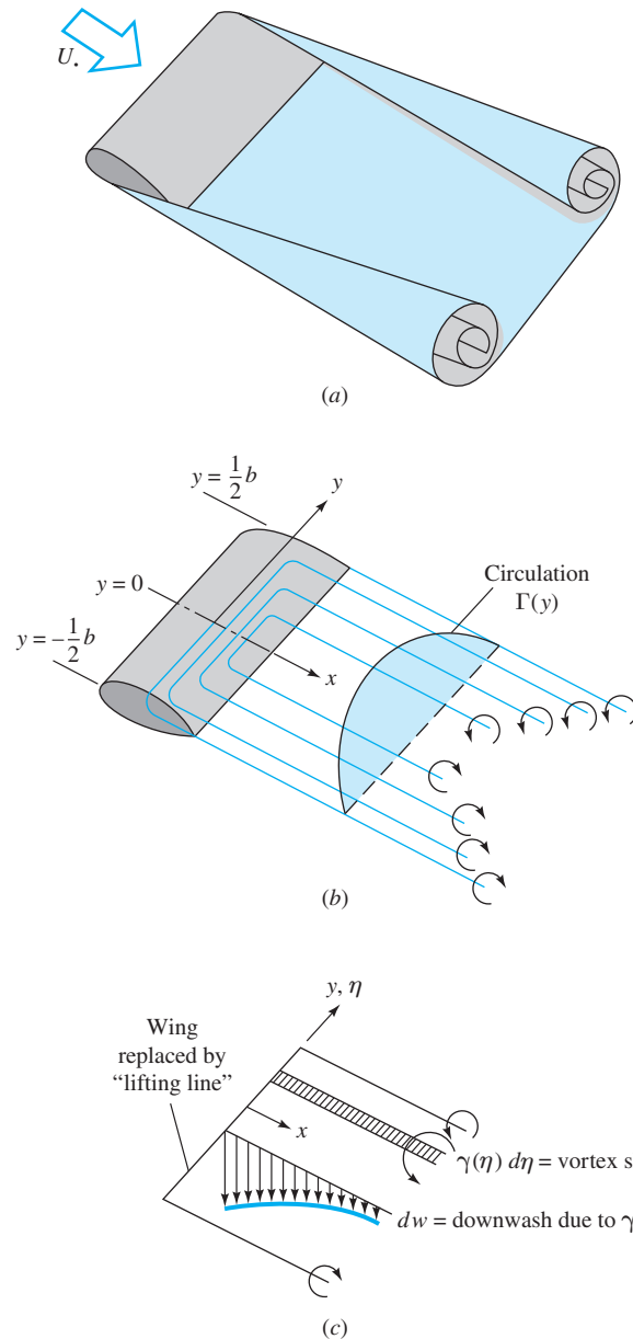
Fig. 8.25 Lifting-line theory for a finite wing: (a) actual trailing-vortex system behind a wing; (b) simulation by vortex system “bound” to the wing; (c) downwash on the wing due to an element of the trailing-vortex system.
