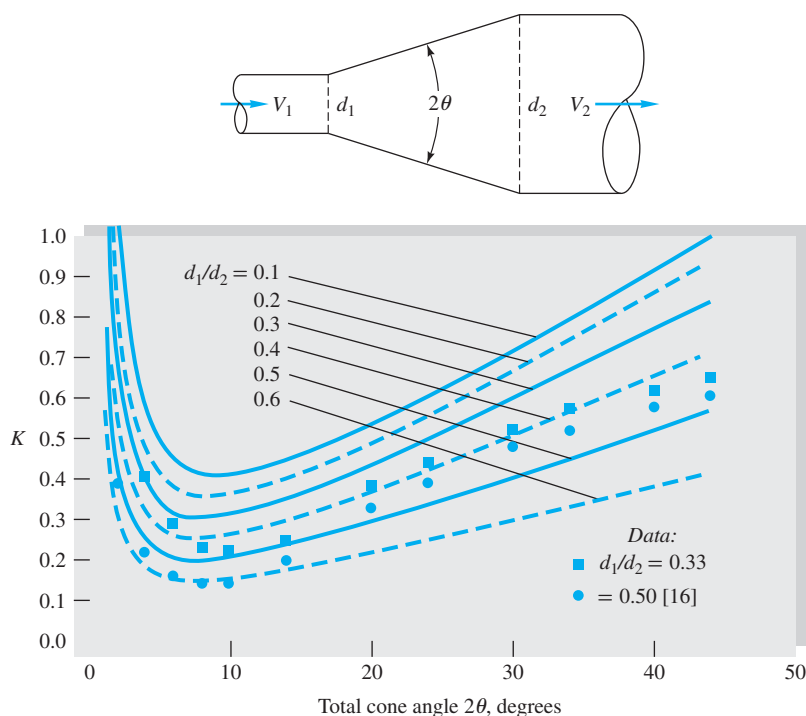
Fig. 6.23 Flow losses in a gradual conical expansion region, as calculated from Gibson's suggestion [15, 50], Eq. (6.79), for a smooth wall.
