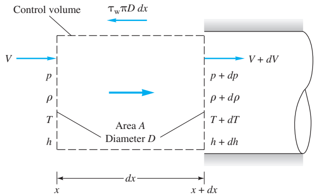
Fig. 9.13 Elemental control volume for flow in a constant-area duct with friction.
