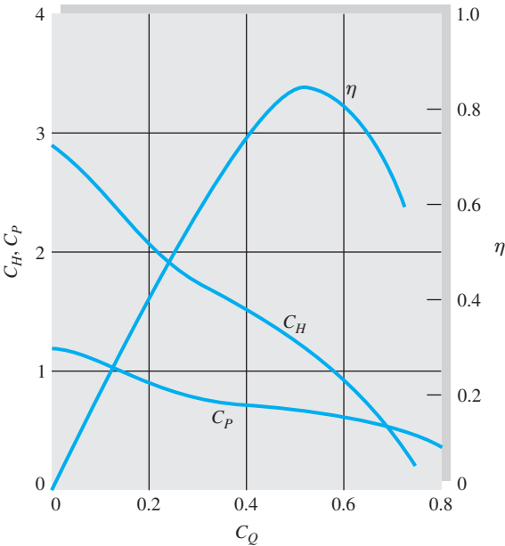
Fig. 11.13 Dimensionless performance curves for a typical axial-flow pump, N_s = 12,000 . Constructed from data given by Stepanoff [8] for a 14-in pump at 690 r/min.
