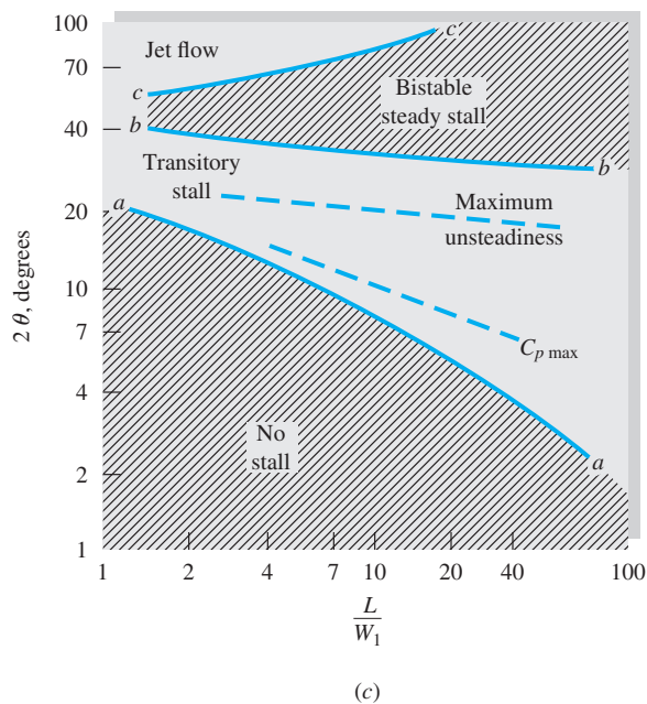
Fig. 6.26 Diffuser geometry and typical flow regimes: (a) geometry of a flat-walled diffuser; (b) geometry of a conical diffuser; (c) flat diffuser stability map. (From Ref. 14, by permission of Creare, Inc.)
