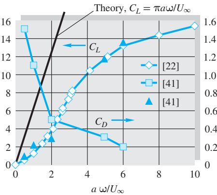
Fig. 8.15 Drag and lift of a rotating cylinder of large aspect ratio at Re_D = 3800 , after Tokumaru and Dimotakis [22] and Sengupta et al. [41].
