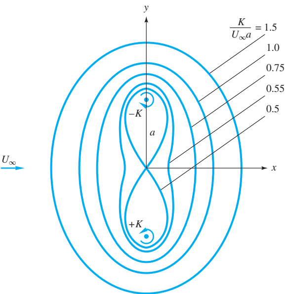
Fig. 8.16 Kelvin oval body shapes as a function of the vortex strength parameter K/(U_\infty a) ; outer streamlines not shown.
