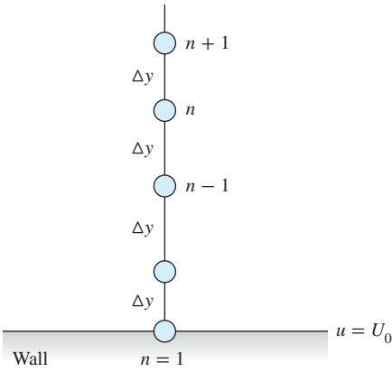
Fig. 8.35 An equally spaced finite difference mesh for one-dimensional viscous flow [Eq. (8.99)].
