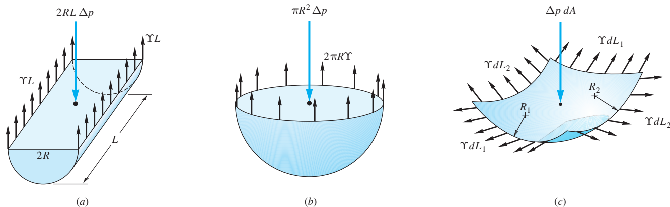
Fig. 1.11 Pressure change across a curved interface due to surface tension: (a) interior of a liquid cylinder; (b) interior of a spherical droplet; (c) general curved interface.
