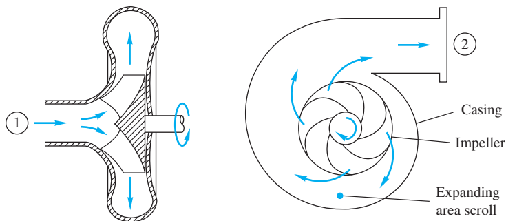
Fig. 11.3 Cutaway schematic of a typical centrifugal pump.
