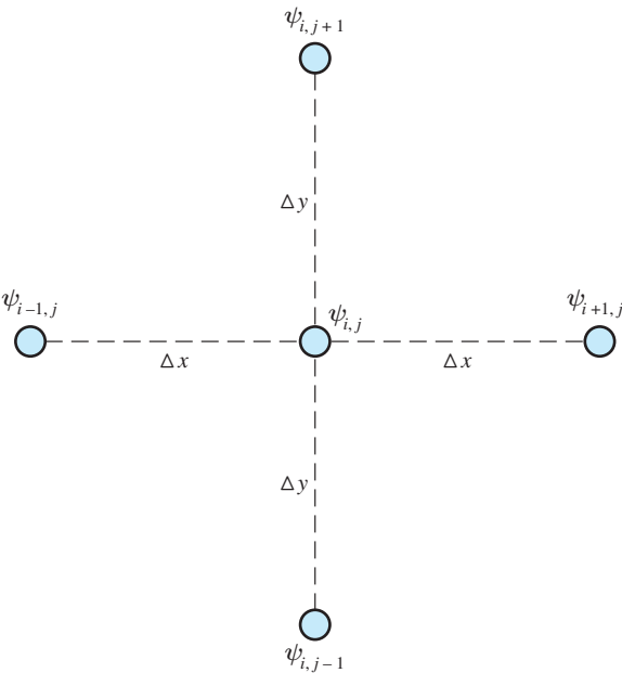
Fig. 8.33 Definition sketch for a two-dimensional rectangular finite difference grid.
