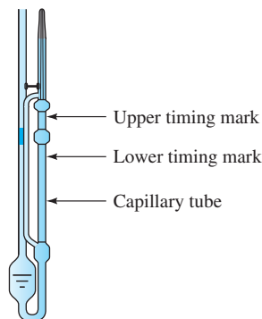
C1.10 The Cannon-Ubbelohde viscometer.
