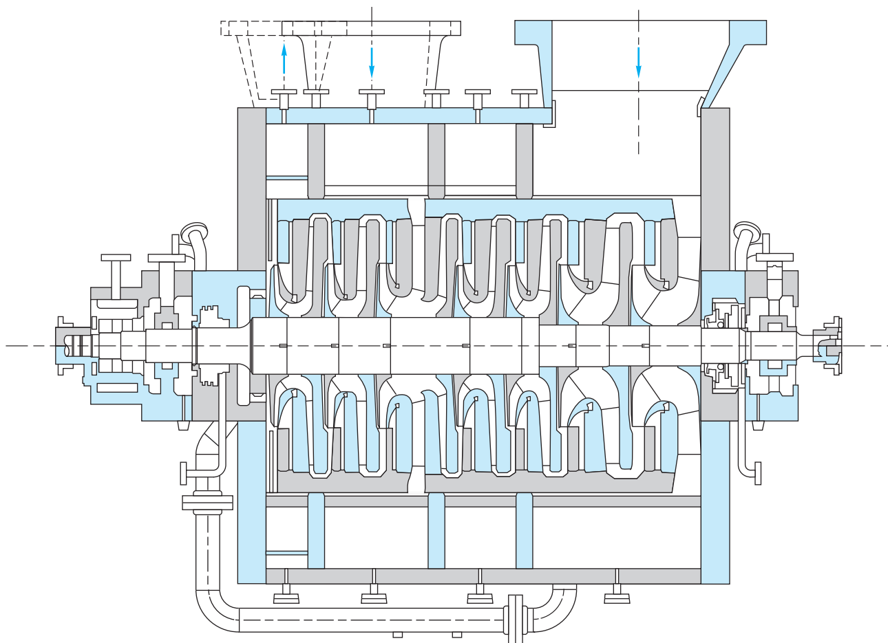
Fig. 11.20 Cross section of a seven-stage centrifugal propane compressor that delivers 40,000 ft 3 /min at 35,000 bhp and a pressure rise of 300 lbf/in 2 . Note the second inlet at stage 5 and the varying impeller designs.
