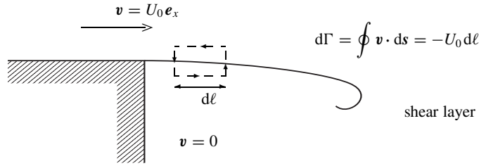
Figure 5.7 Circulation in the shear layer
