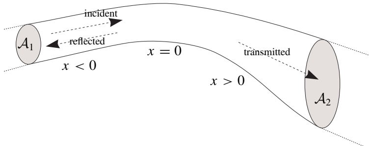
Figure 8.8 Duct junction.
