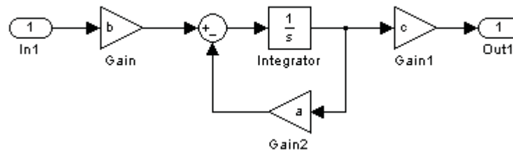
Figure 10.2 Diagram of Model for One State Variable.
