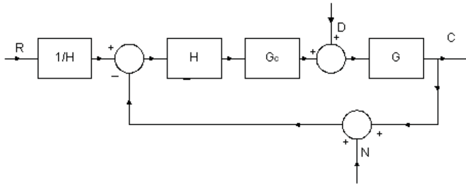
Figure 5.2 Equivalent block diagram to Figure 5.1.
