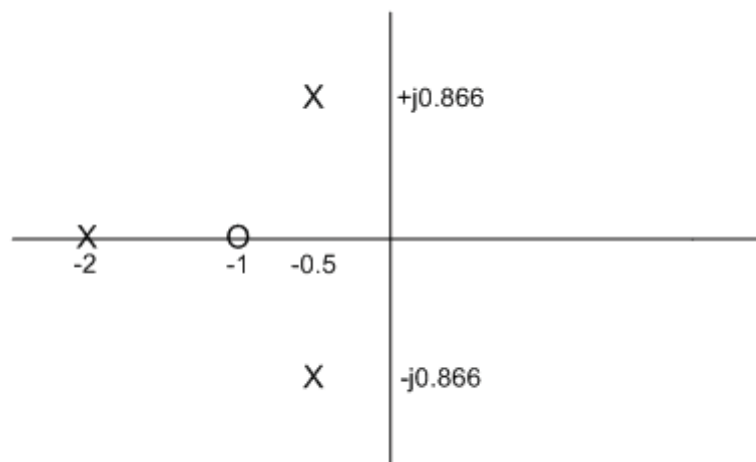
Figure 2.1 Zero-pole plot.
