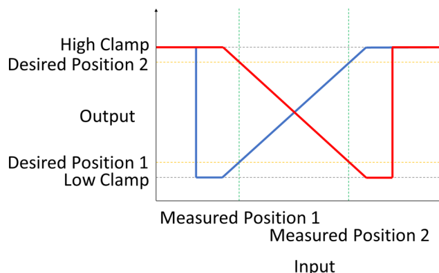
Figure 1: Throttle Position
