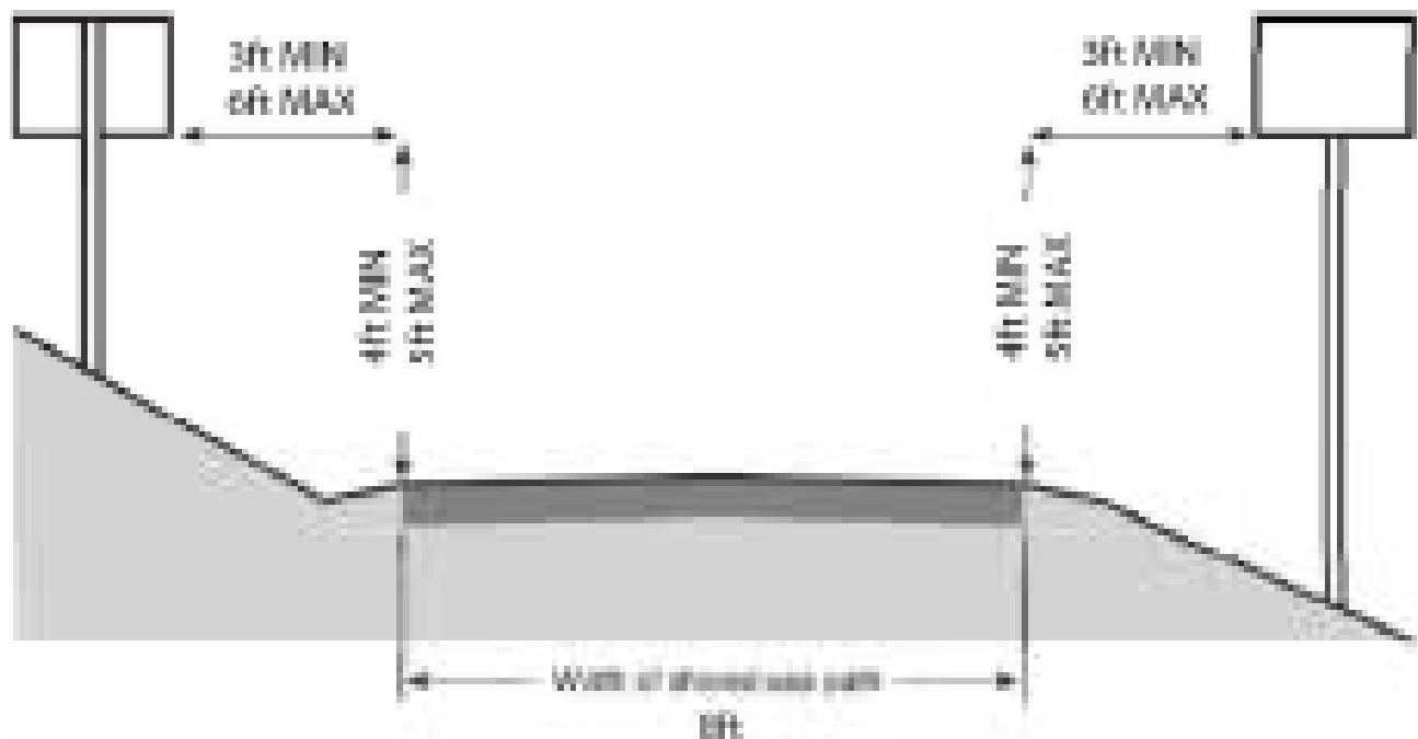
Figure 5 12 Signage Placement
