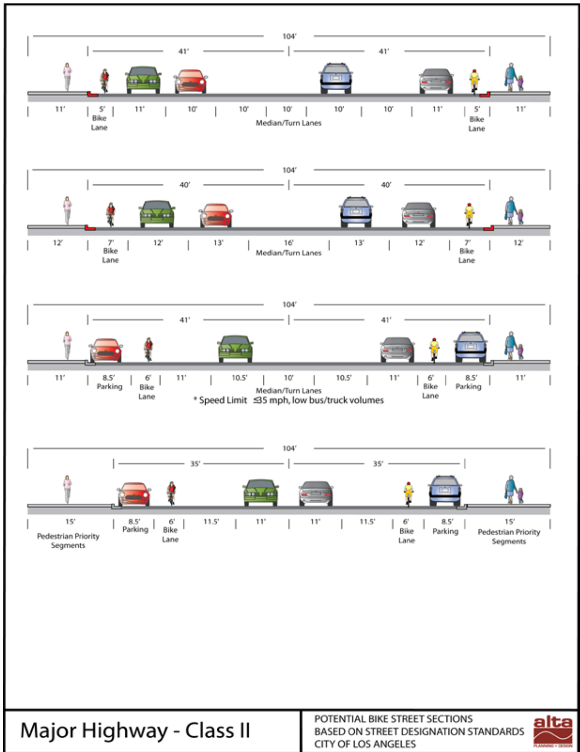
Figure 5-5. Major Highway - Class II - Complete Streets
