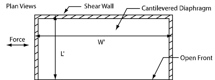
Figure 4A Examples of Open Front Structures
