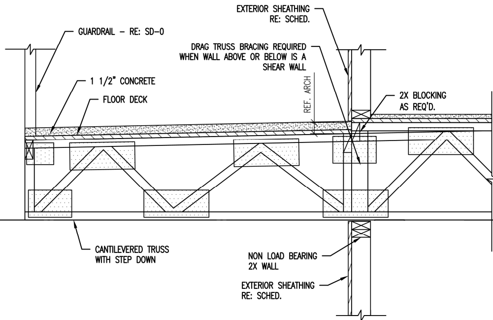
Cantilever Truss – Sloping Top Chord Balcony Framing
