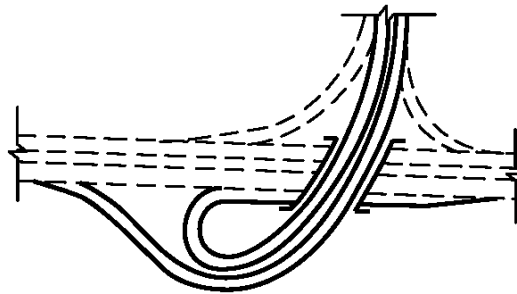
Loop and Semidirectional Ramp
