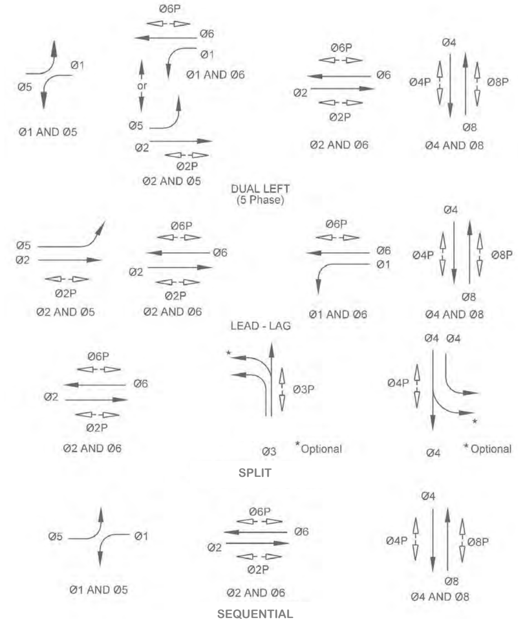
Figure 41-1 | Left Turn Movement Signalization Methods
