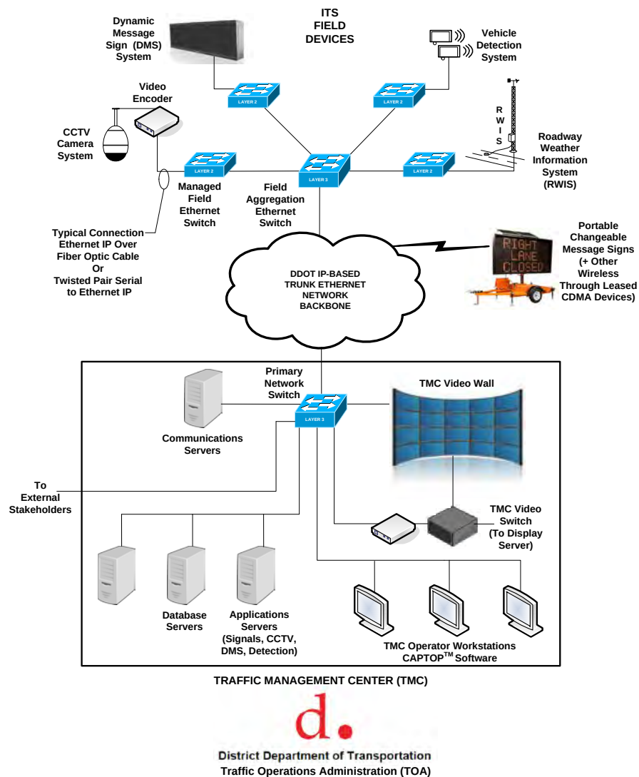
Figure 42-2 | ITS System-Level Diagram and Network Design
