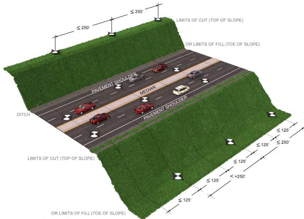
Figure 26-4 | Example of Soil Test Boring Layout for a Four-Lane Road Constructed over Embankment and/or Cut Slope Higher Than 25 Feet
