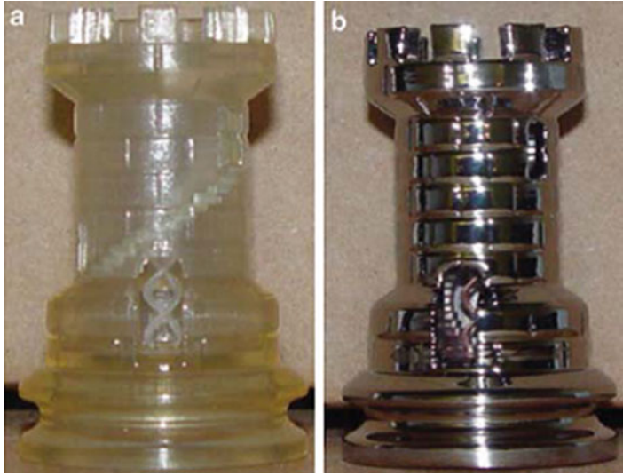
Fig. 14.10 Stereolithography part (a) before and (b) after chrome plating (Courtesy of Artcraft Plating)
