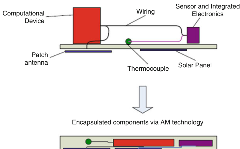
Fig. 9.18 Schematic illustrating the creation of a smart structure using UAM
