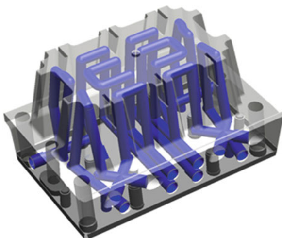
Fig. 18.5 A tool insert design, showing the location of conformal cooling channels
