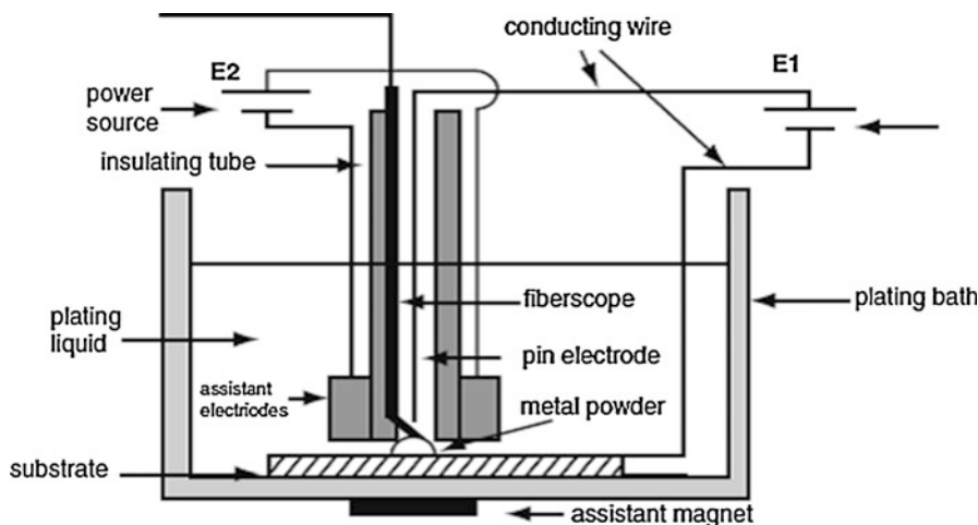
Fig. 11.10 Schematic of an electrochemical liquid deposition system [22] (MATERIALS & DESIGN by Zongyan He, Jack G. Zhou and Ampere A. Tseng. Copyright 2000 by Elsevier Science & Technology Journals. Reproduced with permission of Elsevier Science & Technology Journals in the format Textbook via Copyright Clearance Center.)
