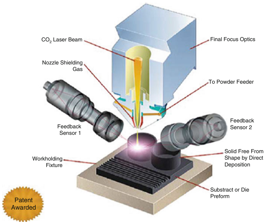
Fig. 10.7 POM DED machine schematic (courtesy POM)
