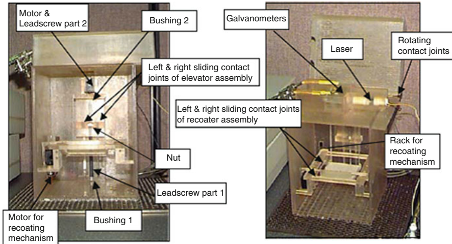
Fig. 17.6 SLA-250 model built in an SLA-250 machine with 11 embedded components
