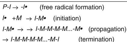
Fig. 4.4 Free-radical polymerization process
