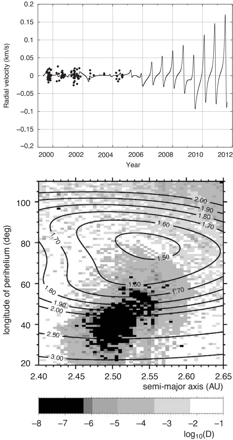
FIGURE 2.19. Top: temporal differences between the radial velocities predicted by the two-Keplerian models and the numerical integration of the system HD 202206 (Correia et al. 2005). Residuals of the CORALIE measurements around the Keplerian solution are displayed as well. Bottom: stability map of the system in a two-parameter plane of the second planet. The minimum \chi^2 of the best-fit solution (lines are iso- \chi^2 contours) is in a chaotic region, close to a stability island corresponding to a 5/1 resonance.
