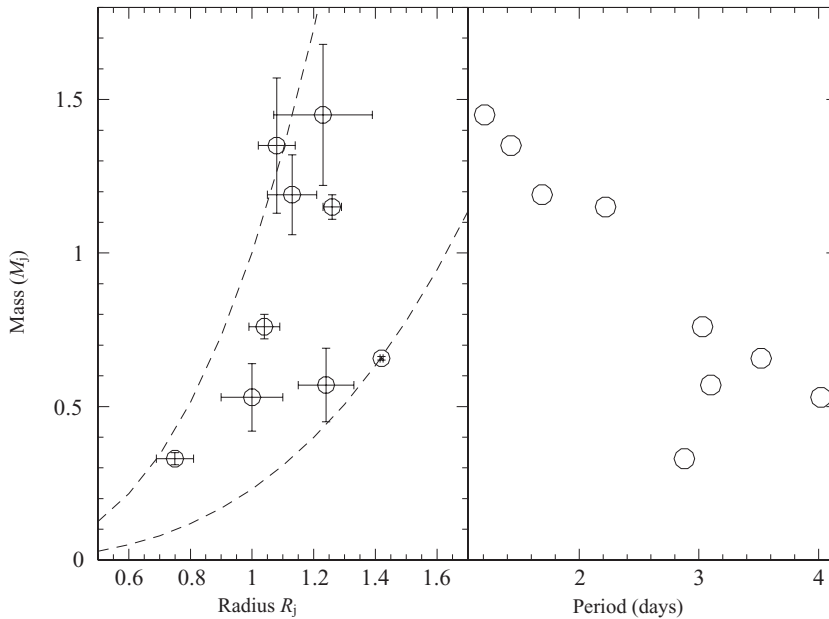
FIGURE 2.22. Mass-radius and mass-period diagrams of transiting planets with radius and accurate mass estimates. In the left panel, the dashed lines indicate isodensity contours of 0.3 and 1.3 \text{g cm}^{-3} .
