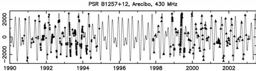
FIGURE 1.1. Time of arrival residuals (in microseconds) of 430 MHz signals from the 6.2-millisecond pulsar PSR B1257 + 12 (from Konacki and Wolszczan 2003) showing that the residuals are dominated by the Keplerian orbits of two planets of actual mass 4.3 (B) and 3.9 (C) Earth-masses (of three in the system, the third being very close to the pulsar). These planets are nearly coplanar (around 50 degrees orbital inclination) and are in actual 3:2 orbital resonance with each other (66.5 and 98.2-day periods; planet A having a period of 25.3 days).
