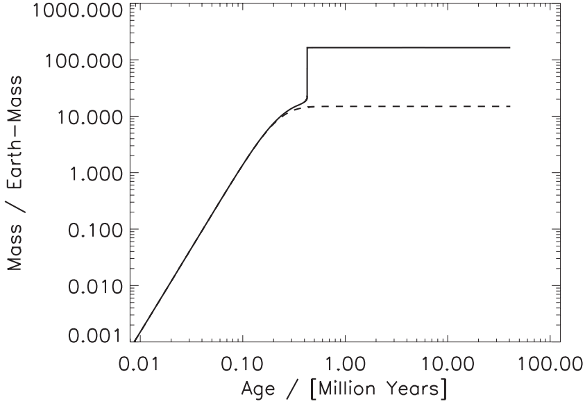
FIGURE 4.4. Total mass (full line) and core mass (dashed line) of a Pegasi planet forming at 0.05 AU from a solar-mass star. The accumulation of a gaseous envelope surrounding a condensable element core that grows by planetesimal accretion is shown for the first 100 million years. The structure of the envelope is calculated dynamically, including time-dependent theory of convection that is calibrated to the Sun and including detailed equations of state and opacities.
