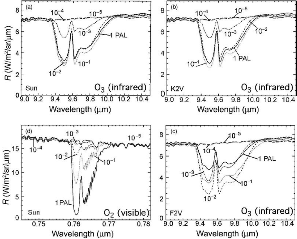
FIGURE 9.4. Variation of the spectral features of O_2 and O_3 with the O_2 level and spectral type of the central star replica. The spectral features produced by O_3 ( 9.6\ \mu\text{m} – frames A, B and C) and O_2 ( 0.76\ \mu\text{m} – frame D) are computed for an Earth replica orbiting a G-, K- or F-star for different O_2 levels (from 10^{-5} to 1 PAL). For the K- and G-stars, the planet–star distance is chosen in order to provide a similar mean surface temperature. The O_2 feature is weakly sensitive to the thermal profile and its shape does not depend on the spectral type. From Segura et al. (2003), courtesy of Antígona Segura and Mary Ann Liebert, Inc.
