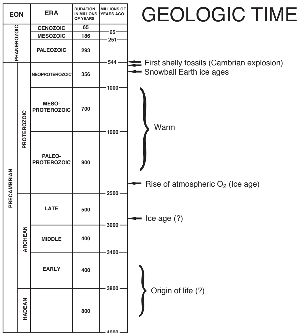
FIGURE 8.1. Geologic timescale showing warm and cold intervals.
