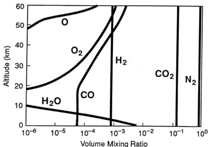
FIGURE 8.9. Vertical profiles of major gases in a weakly reduced prebiotic atmosphere. The assumed surface pressure is 1 bar. The \text{H}_2 mixing ratio is determined by balancing the volcanic outgassing rate with the diffusion-limited escape rate of hydrogen to space. From Kasting 1993.
