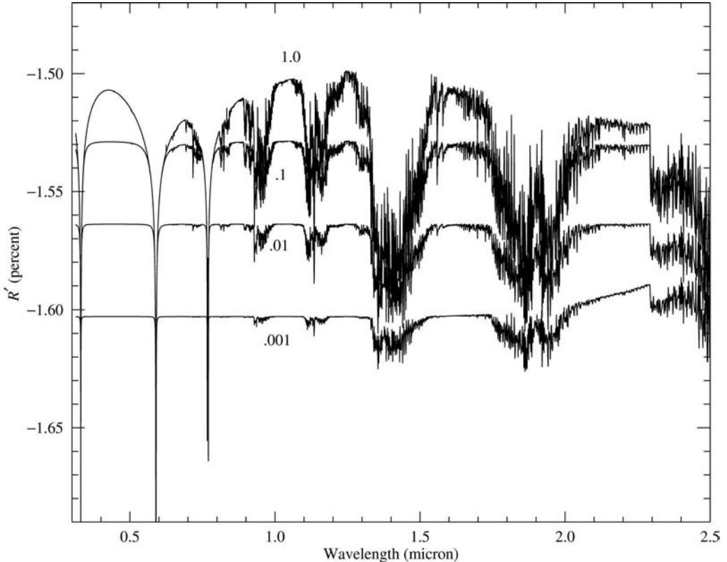
FIGURE 3.8. Theoretical visible and near-infrared transit spectra of HD 209458b, computed assuming a range of cloud heights. Deep bands of \text{H}_2\text{O} and CO can be seen, as well as the pressure-broadened resonance lines of Na and K. The contrast of all these features depends upon the cloud height, decreasing as the height of the cloud tops increases (Brown, 2001).
