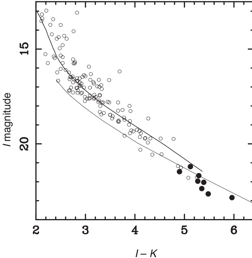
FIGURE 6.4. The Pleiades brown dwarf sequence in the I versus I - K diagram. The new candidate L-type brown dwarfs from the survey by Bihain et al. (2006) are marked with filled circles. The upper solid line is the DUSTY model 100 My isochrone from Chabrier et al. (2000). The line below shows the location of field L-dwarfs shifted to the distance of the Pleiades.
