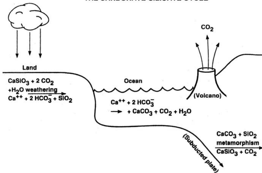
FIGURE 8.3. Diagram illustrating the carbonate–silicate cycle.
