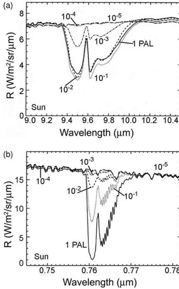
FIGURE 8.11. Calculated shape of the ozone 9.6- \mu\text{m} absorption band (a) and the \text{O}_2 0.76- \mu\text{m} band (b) for the atmospheric models shown in Figure 8.10. From Segura et al. 2003.
