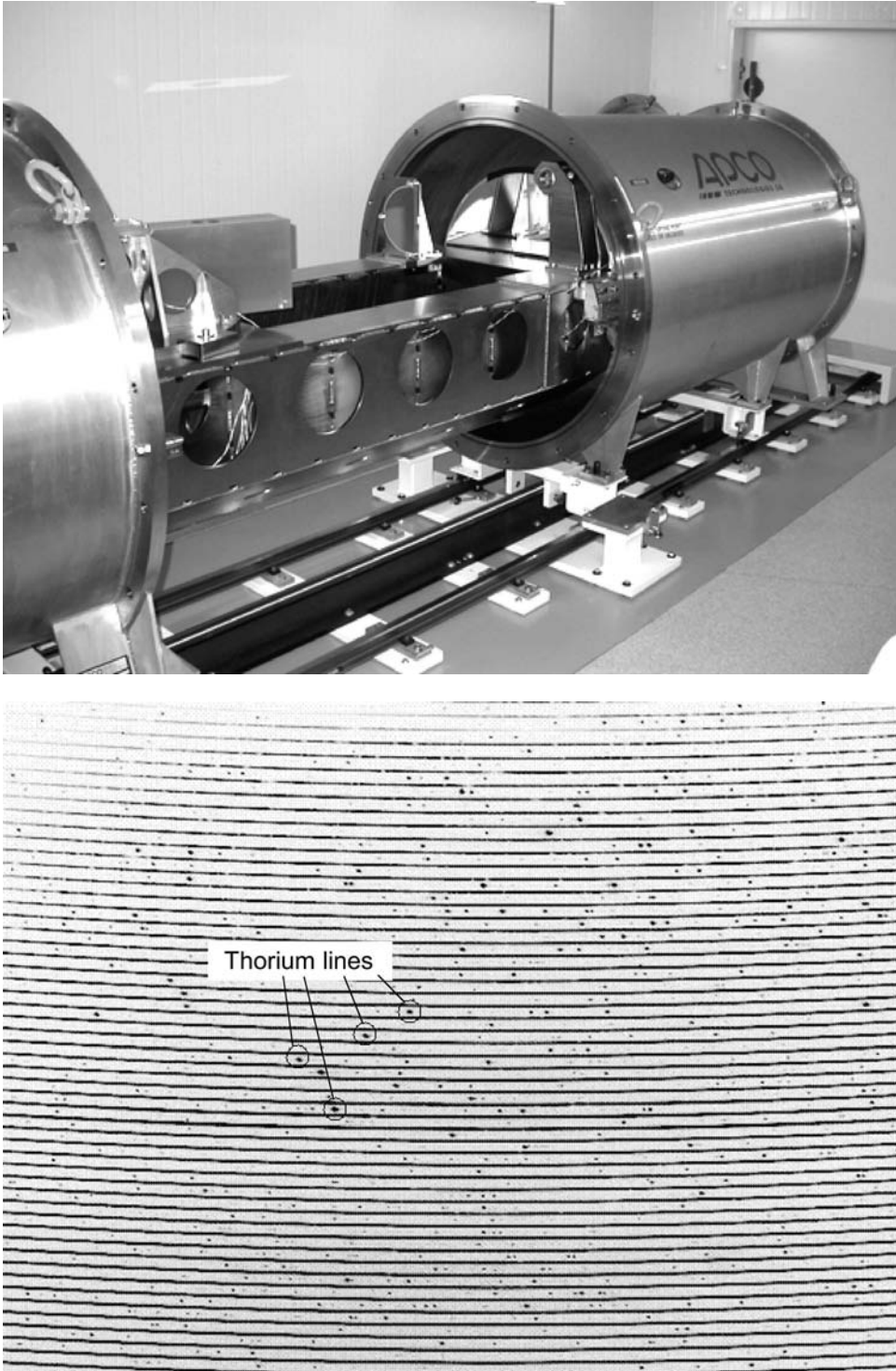
FIGURE 2.4. Top: view of the HARPS-spectrograph grating inside the vacuum tank. Bottom: raw CCD image obtained with HARPS, with the alternate orders of a star and the lamp spectra.
